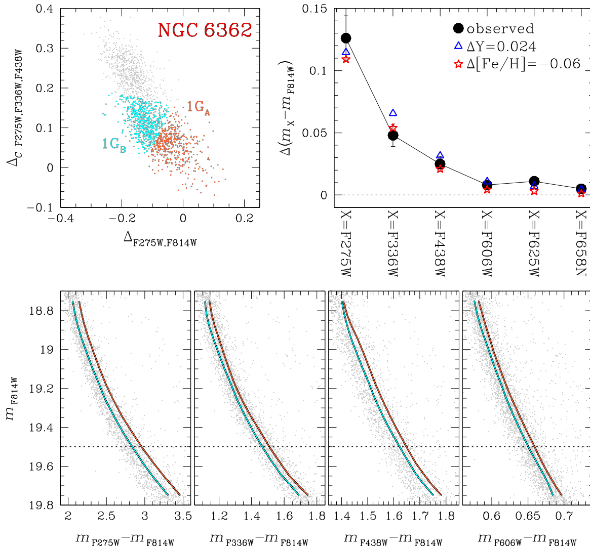
Figure 4. This figure illustrates the procedure used to derive the colour differences between the two sub-groups of 1G_A and 1G_B stars for NGC 6362. The upper-left panel reproduces the ChM of MS stars with the orange and cyan points that identify 1G_A and 1G_B stars, respectively. The lower panels show the m_{F814W} versus m_X - m_{F814W} CMDs where X = F275W, F336W, F438W, and F606W (the same has been done for F625W and F658N filters) in which the fiducial lines obtained for 1G_A and 1G_B are plotted in orange and cyan. In each panel, the horizontal dotted line corresponds to the reference F814W magnitude at which we calculate the colour separation, \Delta(m_X - m_{F814W}) . The upper-right panel shows the \Delta(m_X - m_{F814W}) calculated at m_{F814W}^{\text{ref}} = 19.5 against the central wavelength of the X filter. The colours inferred from the best-fitting synthetic spectra are overplotted with blue triangles and red starred symbols (see text for details).
