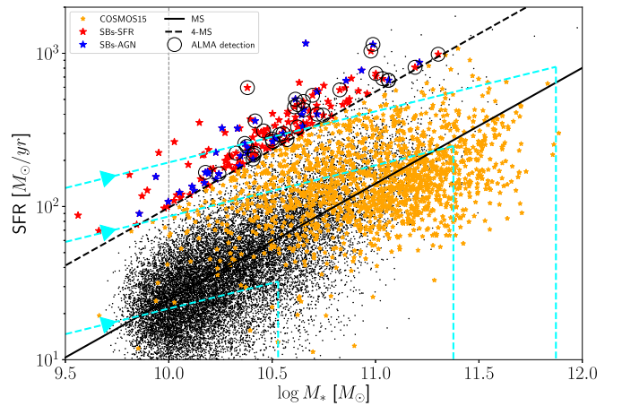
Figure 1. Sample selection in the SFR- M_* plane for the COSMOS field at 1.5 < z < 2.5 . Orange stars mark the original Herschel sample. Blue and red stars show the position of SBs-AGN and SBs-SFR, respectively (see Section 2.1). Black open circles indicate the SB sources with an ALMA detection. Black dots are star-forming BzK (Daddi et al. 2007). We report as dashed cyan lines evolutionary tracks of galaxies (Lapi et al. 2018) starting with different initial SFR and final total M_* (time follows the arrows direction, see the discussion in Section 6.2). The vertical black dashed line marks the mass limit of our SBs selection (see the text for details).
