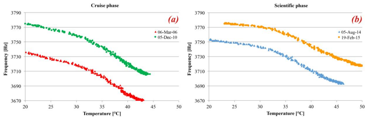
32 Fig. 9: QCM5 frequency vs. temperature during the active heating process performed during 33 the Rosetta cruise (a) and scientific (b) phases. The trend of these curves is in accordance with 34 typical behaviour for AT-cut QCM (Sauerbrey, 1959) and comparable with the frequency vs 35 temperature curves provided by the QCM manufacturer. 36
