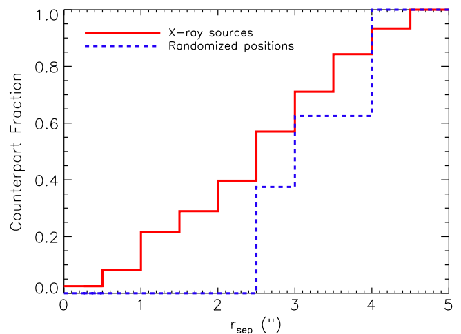
Figure 10. Similar to Figure 4, but for the X-ray and Herschel nearest-neighbor matches, with 121 counterparts and 8 spurious associations within r_{\text{search}} = 5'' . Just as Figure 9 shows, the matching between the X-ray source list and FIRST, most of the spurious matches occurs at higher values of r_{\text{sep}} .
