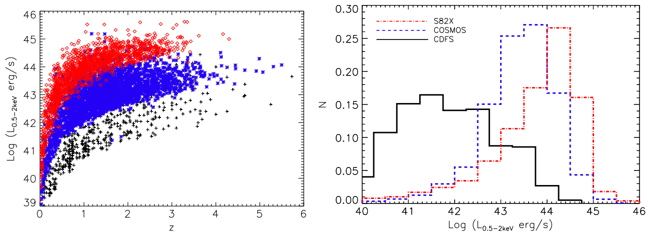
Figure 14. Left: K -corrected (rest-frame) soft-band (0.5–2 keV) luminosities as a function of redshift for the Stripe 82X (red diamonds; Civano et al. 2015; Marchesi et al. 2015), COSMOS-Legacy (blue asterisks; Civano et al. 2015; Marchesi et al. 2015), and CDFS (black crosses) sources. At every redshift, an increase in survey area preferentially identifies higher-luminosity sources. Right: normalized distribution of k -corrected soft-band luminosities for Stripe 82X compared with COSMOS and CDFS: the wide-area coverage of Stripe 82X which probes a large effective volume of the universe, enables the rare, highest luminosity quasars to be uncovered, complementing the parameter space explored by small- to moderate-area surveys. In both plots, only the sources identified with redshifts are plotted, representing 30% of the Stripe 82X sample (which currently has only spectroscopic redshifts) and 91% and 96% of the CDFS and COSMOS-Legacy sample, respectively, where both spectroscopic and photometric redshifts are available.
