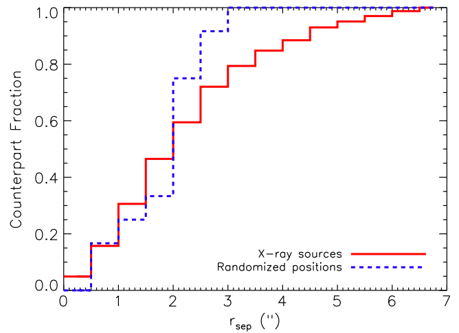
Figure 8. Similar to Figure 4, but for the X-ray/ GALEX matches to the NUV band, where 572 counterparts and 12 matches to randomized positions lie above R_{\text{crit}} .
