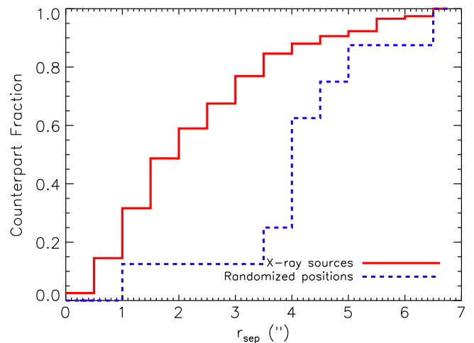
Figure 9. Similar to Figure 4, but for the X-ray and FIRST nearest-neighbor matches, with 116 counterparts and eight randomized matches found within r_{\text{search}} = 7'' . Here, many of the spurious associations are found at higher separation distances due to the low number density of radio and X-ray sources.
