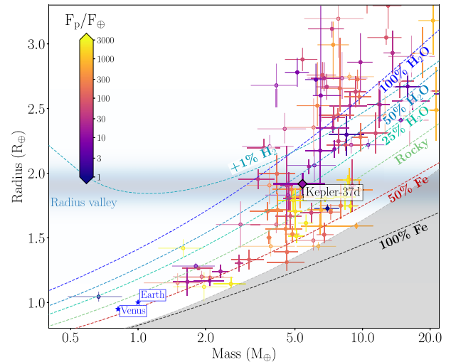
Figure 10. Mass–radius diagram for exoplanets with masses and radii measured with better than 30 per cent precision, colour coded according to their incidental flux (Earth units). Kepler-37d is indicated with a large diamond. The dashed coloured lines represent theoretical mass–radius curves for various chemical compositions according to Zeng et al. (2019). The shaded grey region denotes the maximum Fe content predicted by collisional stripping (Marcus et al. 2010). Data taken from the The Extrasolar Planets Encyclopaedia ( http://exoplanet.eu/catalog/ ) on 2021 March 26.
