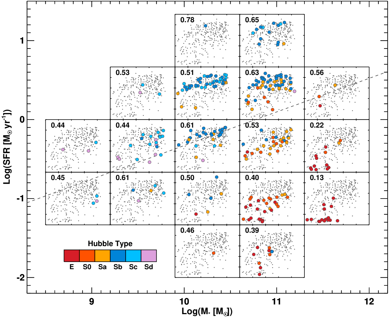
Fig. 7. \lambda_{Re}-\epsilon relation as a function of location in the star-formation rate versus total stellar mass ( M_* ) relation for the CALIFA galaxies. Each panel shows the complete sample highlighting in color the ones belonging to each specific SFR– M_* bin. The number in each subpanel gives the V_{max}^{-1} -weighted \lambda_{Re} average for the highlighted galaxies in that bin. The dark gray dashed line in the SFR versus M_* on the right marks the division between the main star-forming sequence and quiescent galaxies from Renzi & Peng (2015) .
