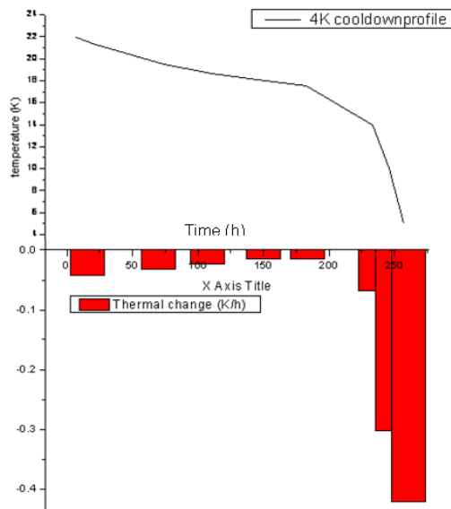
Figure 5 4K stage cooldown in CSL ( top graph) against its slope in K/ h ( bottom graph). X axis represents time in hours.
