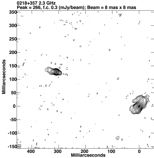
Figure 2. Stacked image of B0218+357 at 2.3 GHz. The beam is plotted on the bottom-left corner. We provide the peak flux density in \text{mJy beam}^{-1} , the first contour (f.c.) intensity ( \text{mJy beam}^{-1} ), which is three times the off-source noise level measured on the image plane and the size of the beam. Contour levels increase by a factor of 2.
