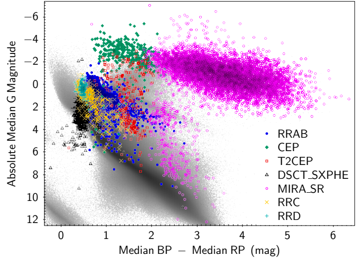
Fig. 7. Colour-absolute magnitude diagram (as absolute median G -band magnitude vs. median G_{BP} – median G_{RP} ) of a selection of classification candidates: fundamental mode (RRAB, blue dots), first-overtone (RRC, orange “x” marks), and double-mode (RRD, cyan “+” marks) RR Lyrae types, classical (CEP, green rhombi) and type-II (T2CEP, red squares) Cepheids, \delta Scuti/SX Phoenicis types (DSCT_SXPHE, black triangles), and Mira/semiregular types (MIRA_SR, magenta circles). Faint outliers typically denote contaminating objects, which in the case of long-period variables, are represented mostly by young stellar objects. All of these sources satisfy the conditions listed in Appendix B of Gaia Collaboration (2019), among which a relative parallax precision better than 20%, with no correction for interstellar or circumstellar extinction or reddening. The background points in grey act as a reference of objects within a radius of 1 kpc from the Sun.
