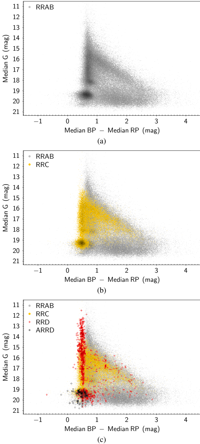
Fig. 8. Colour-magnitude diagram (as median G -band magnitude vs. median G_{BP} - median G_{RP} ) of the RR Lyrae classifications. The three panels show the fundamental mode (labelled RRAB, grey dots), first-overtone (labelled RRC, orange dots), and (anomalous) double-mode (labelled ARRD/RRD, black circles/red crosses) RR Lyrae subtypes, cumulatively, in panels a-c , respectively. See text for the explanation of the main features.
