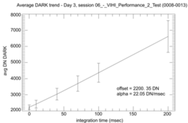
Fig. 40: The VIHI dark-current signal vs. integration time.
