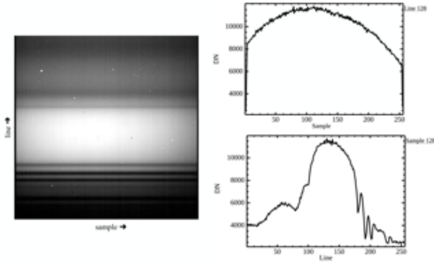
Fig. 36: VIHI internal calibration lamp signal. The image of the Focal Plane (left) shows spectral information in the vertical direction and spatial information in the horizontal direction. Two profiles show spatial variability (top right) across the FoV and the spectrum (bottom right) from 400 nm (band 255) to 2000 nm (band 0).
