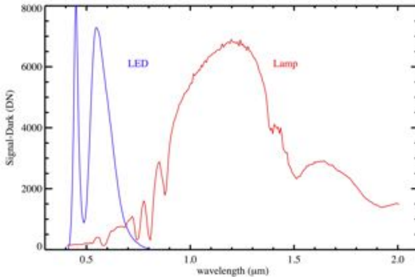
Fig. 28: The VIHI internal calibration unit reference spectral signals from the LED and IR lamp as measured at boresight ( s = 128 ). Note the position of the absorption features on the LED and IR Lamp spectra used to check the spectral response stability. From Filacchione et al. (2017) .
