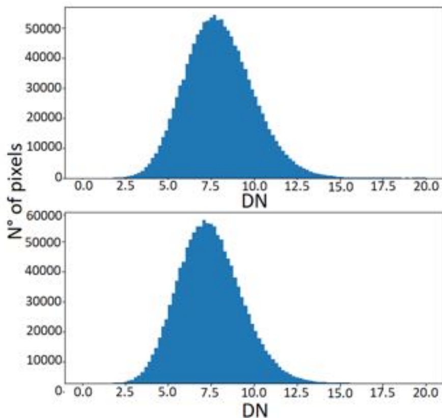
Fig. 34: RON histograms averaged over 10 acquisitions, at the minimum integration time (top) and 48 \mu\text{s} (bottom).
