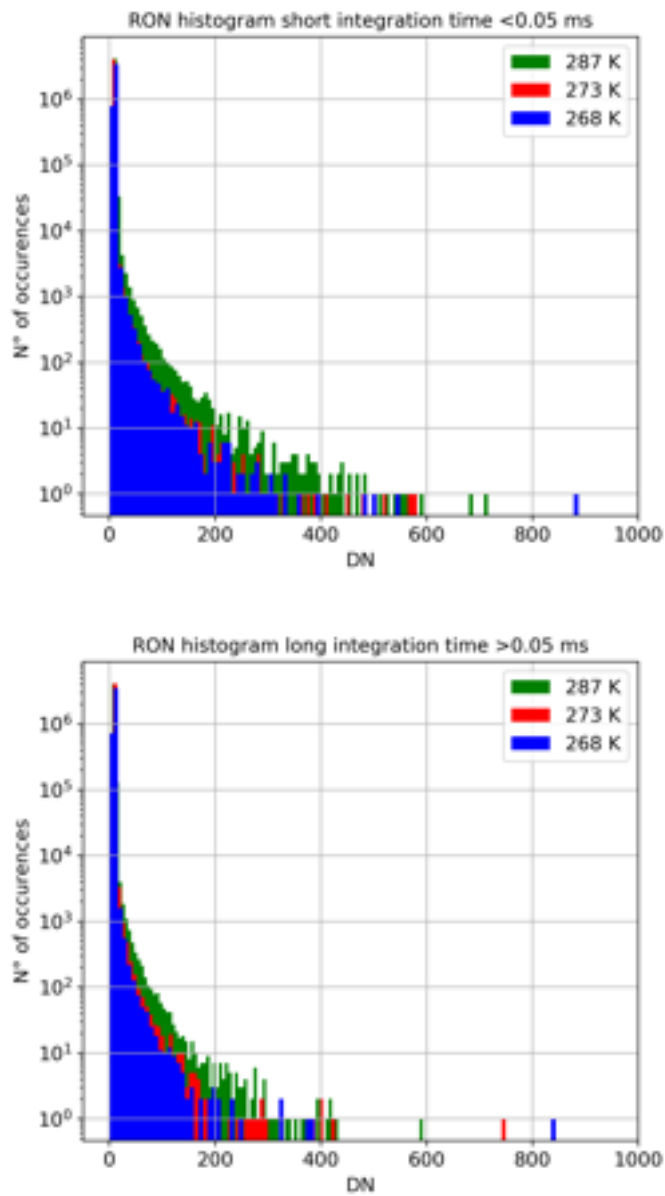
Fig. 14: Histograms of the RON distribution for the whole detector for IT < 0.05 ms (top) and IT > 0.05 ms (bottom). The distributions are reported for the 3 different temperatures.
