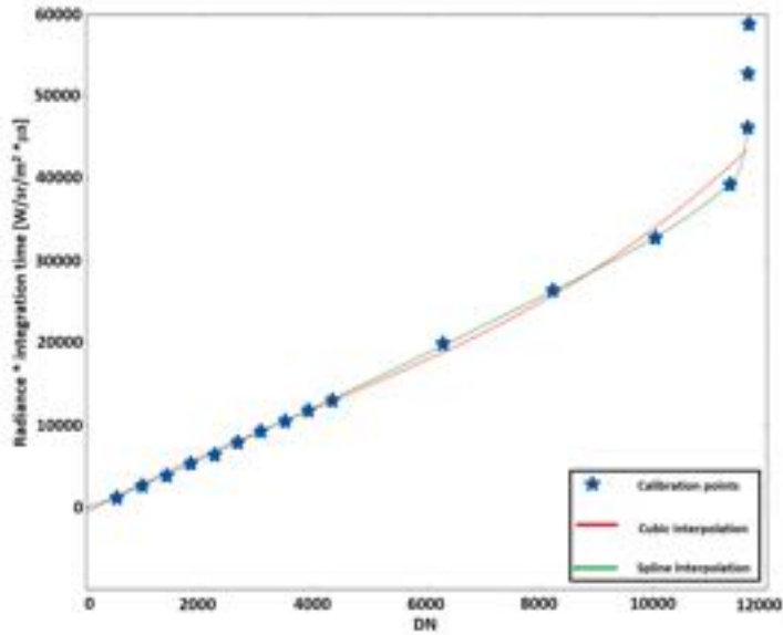
Fig. 15: Radiometric calibration curve for the panchromatic filter. The plot shows the measurements obtained with a calibrated source at different integration times. However, a linear region of the detector can be identified. We tried to work on the data with more complex fitting law to extend the dynamical range. We obtained good results using spline fitting. The same approach has been used for the 4 broad-band filters.
