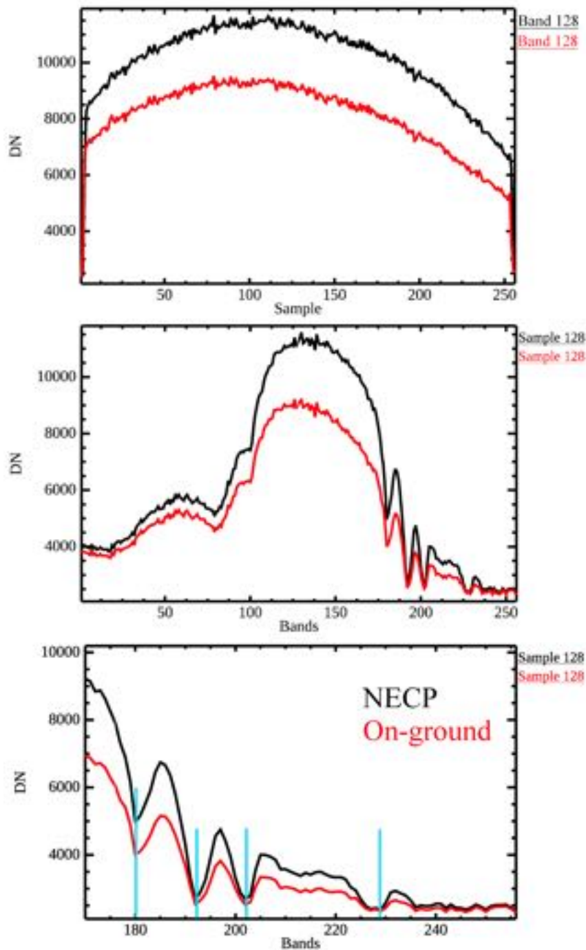
Fig. 37: The VIHI spectral response verification. The comparisons between the NECP tests (top and middle, black lines) and the on-ground ones (red lines). The two profiles show spatial variability (top) across the FoV and the spectrum (central), from 400 nm (band 255) to 2000 nm (band 0). A spectral profile zoom above the constant position of the Didymium filter absorption bands is also shown before and after launch (bottom).
