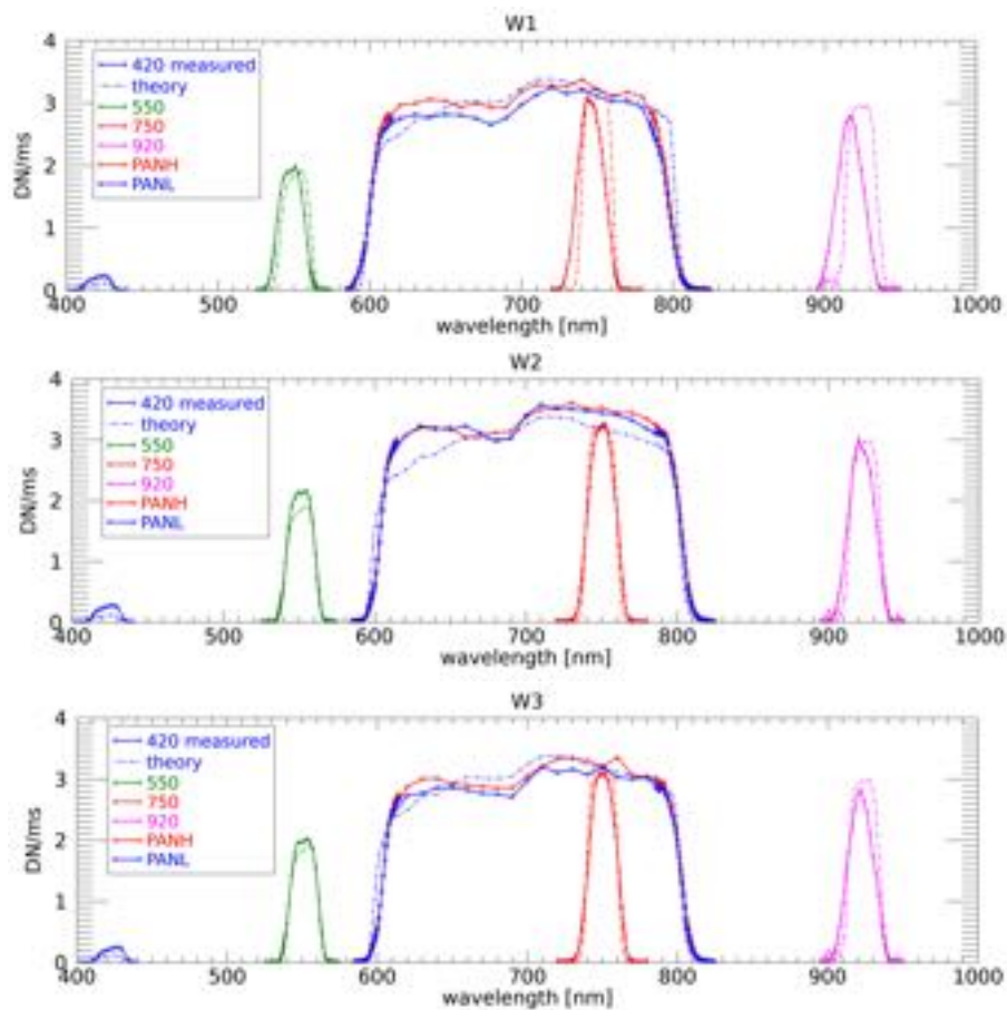
Fig. 20: Comparison between the flux per unit of time detected by the CMOS sensor and those estimated with the theoretical transmittance curve. The titles "W1", "W2", and "W3" refer, respectively, to the left-side, central, and right-side sub-windows. The solid lines refer to the measured flux per unit of time, whereas the dashed lines represent the values obtained with the theoretical transmittance curve.
