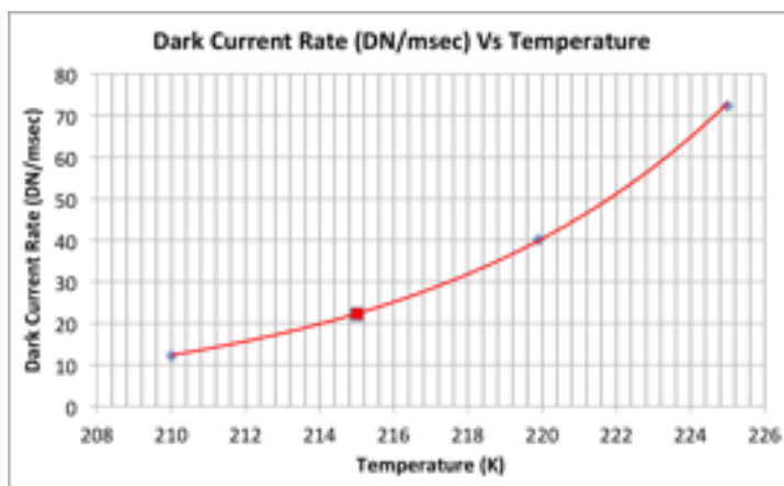
Fig. 41: The VIHI dark-current rate vs. focal-plane temperature. The in-flight value is reported in red, while the cyan losanges represent the ground calibration measurements.
