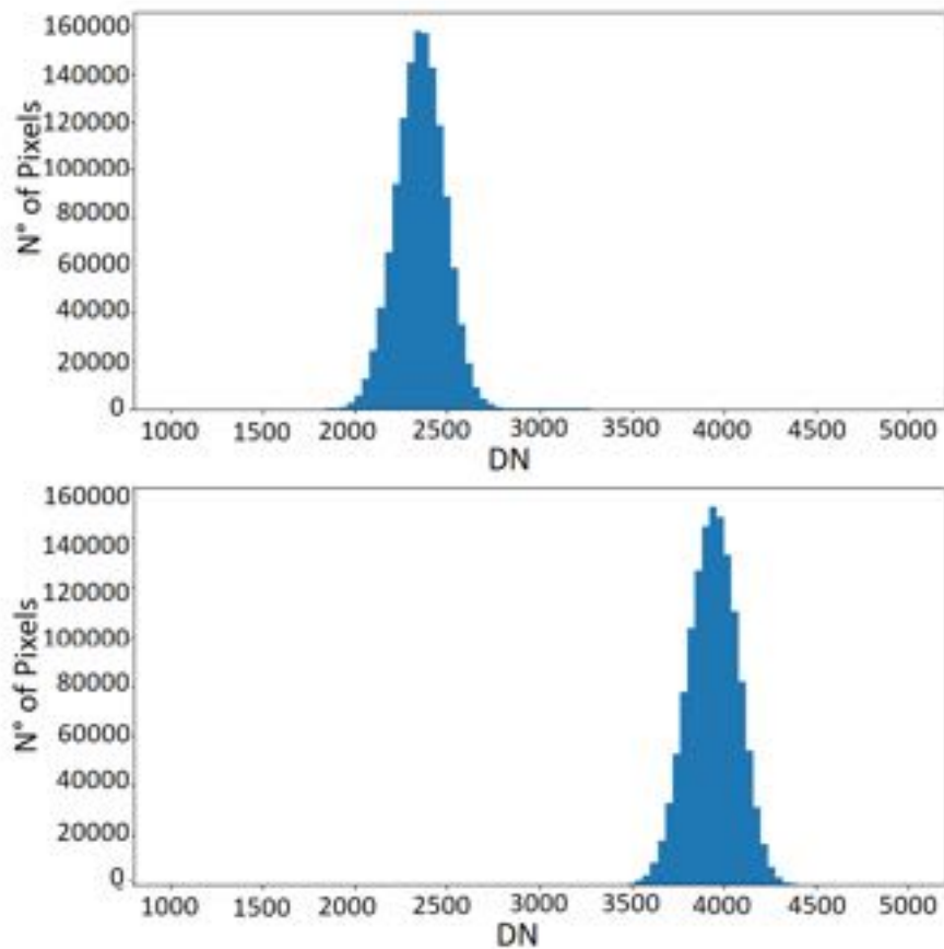
Fig. 33: FPN histograms averaged over 10 acquisitions, at the minimum integration time (top) and 48 \mu\text{s} (bottom).
