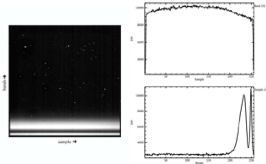
Fig. 38: The VIHI internal calibration LED source signal measured during commissioning: the signal on the detector frame (left, spectral information along the vertical direction and spatial information along the horizontal direction) and the spatial variability across the FoV (top right) and the spectrum (bottom right) from 400 nm (band 255) to 2000 nm (band 0).
