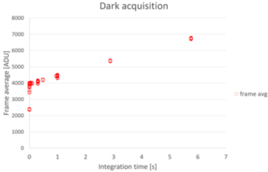
Fig. 32: Panchromatic DC trend, the average value of the frames acquired at different integration times. For each exposure time, several measurements (open circles) are reported, because 10 images have been acquired. The data are compatible with the behaviour already observed during ground calibration, including the peculiar trend for IT < 0.05 ms (see Figure 12).
