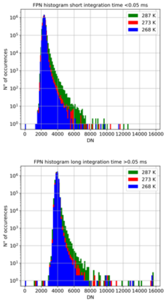
Fig. 13: FPN histograms. The distributions of the spatial non-uniformity of the pixel level for IT <math>< 0.05\text{ ms}</math> (top) and IT <math>> 0.05\text{ ms}</math> (bottom).
