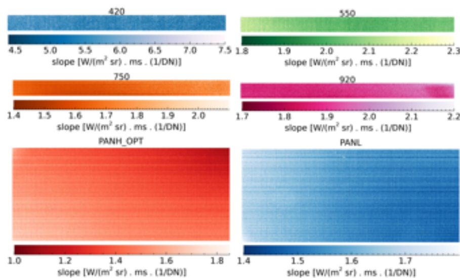
Fig. 18: Mean values of the slopes of the radiometric function in the linearity range for each filter of the STC detector. For each filter, two stripes are depicted. The upper stripe corresponds to the area covered by the filter on the detector, where the color shows the calculated values of the slope. The bottom stripe corresponds to the color coding.
