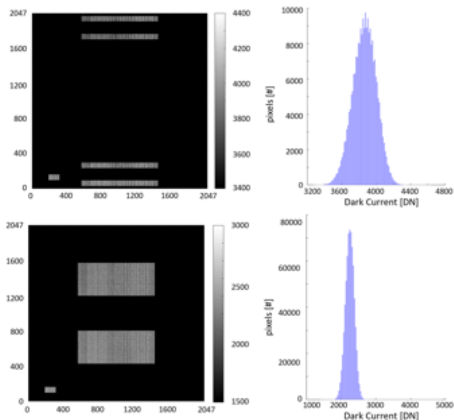
Fig. 35: Two examples of acquisition for STC during the NECP: the global mapping mode (top) and the color mode (bottom). The STC detector is shown on the left and the dark signal distribution on the right. In both cases, the histogram has a width around 800 DN corresponding to a foreseen standard deviation of 135 DN.
