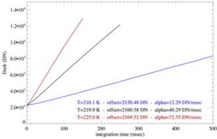
Fig. 26: Trends of the VIHI median dark-current values measured on the full detector for the temperature cases T_{cold} = 210.1 K, T_{nominal} = 219.9 K, and T_{warm} = 225.0 K. The offset and dark-current rate (alpha) as a function of integration time are calculated by means of a linear fit are shown for each case. Detector's saturation occurs at about 13200 DN. From Filacchione et al. (2017) .
