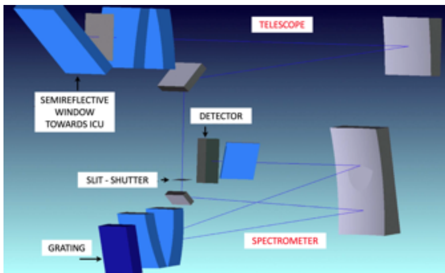
Fig. 7: VIHI Optical Layout. (Courtesy of Leonardo SpA)
