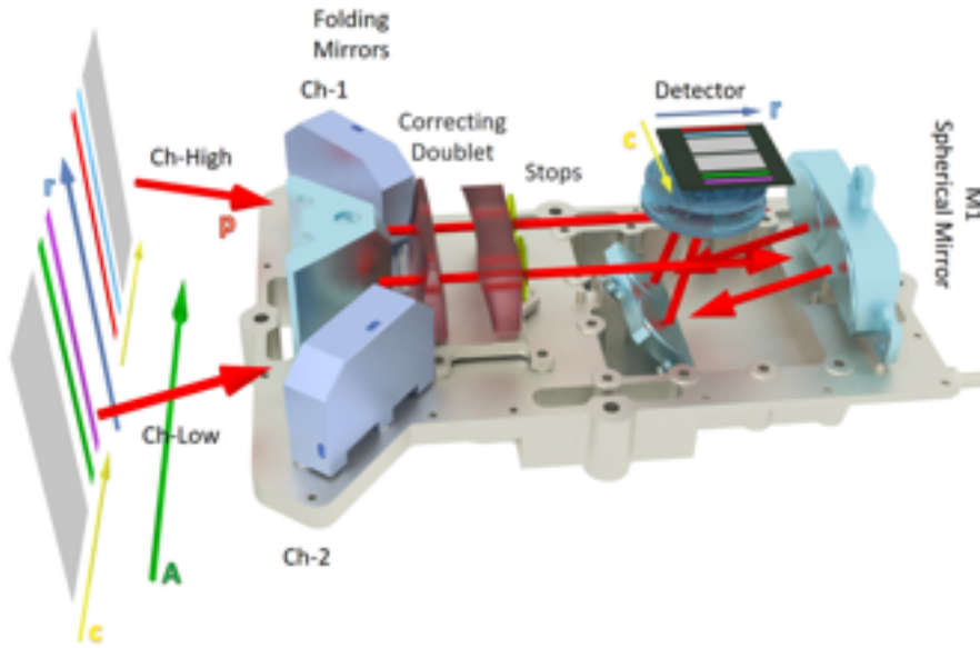
Fig. 4: STC schematic optical layout. From left to right: the on-ground FoV for all the filter frames is shown together with the projected directions of the detector rows (r) and columns (c). The green (A) and blue arrows (r) show, respectively, the along-track and cross-track directions. The optical path (p), through the camera to the detector, is depicted in red. On the detector, the directions of columns (c) and rows (r) are shown. The AT direction, A in green, changes at perihelion and aphelion, when the flip of the MPO will occur.
