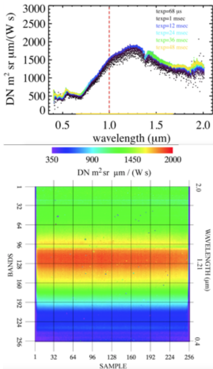
Fig. 27: The VIHI responsivity at sample = 128 (top) for integration times between 68 \mu\text{s} and 48 ms and the VIHI responsivity array (bottom) as derived for the integration time t = 10 \text{ ms} . From Filacchione et al. (2017) .
