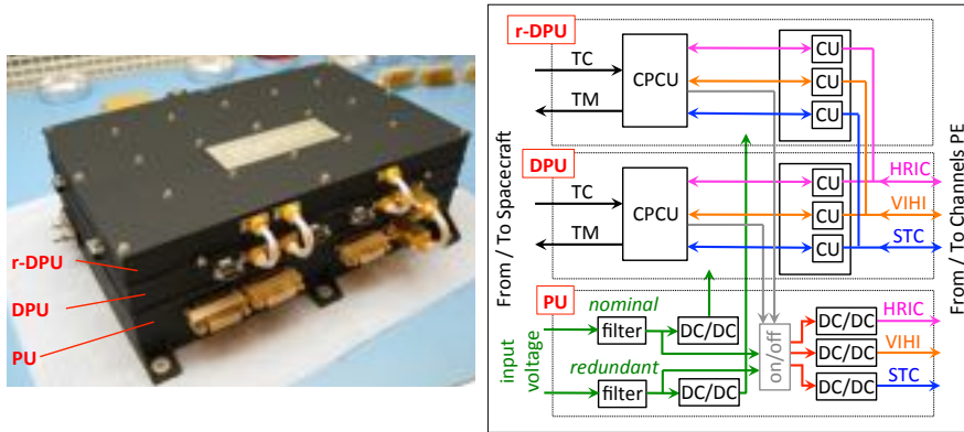
Fig. 9: Main Electronics. The ME qualification model (left) showing the three electronics boards within their housing (from top to bottom, redundant DPU “r-DPU”, DPU, and PU) and a simplified ME functional Block Diagram (right). See text for acronyms.
