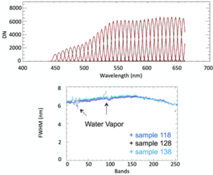
Fig. 24: Signal of the monochromator (top, black lines) acquired during the spectral scan at boresight (sample s = 128 ) and spectral response function (red lines) derived from a Gaussian fit for the spectral range of 440 \leq \text{bands} \leq 660 nm. Variability of the spectral response width (bottom) at three samples along the spectral axis. Water vapor residuals are visible at bands \approx 20 and \approx 90 . Adapted from Altieri et al. (2017) .
