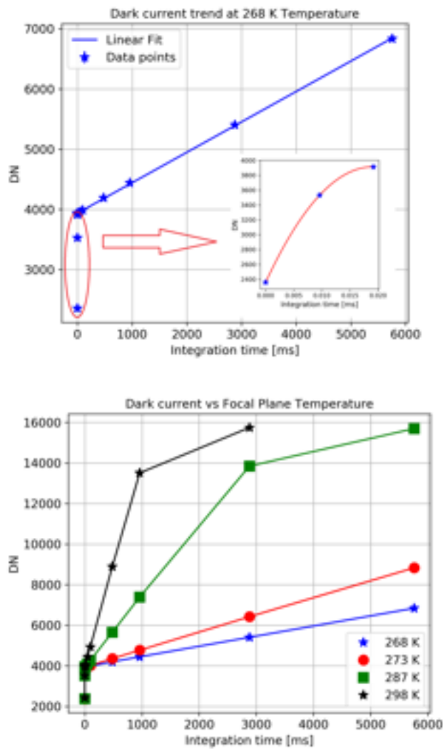
Fig. 12: DC behaviour. The top panel shows the double rate of the DC, for very short IT < 0.05 ms, we obtain a parabolic trend, while a linear trend is measured for IT > 0.05 ms. The bottom panel reports the dependence of the DC as a function of the temperature.
