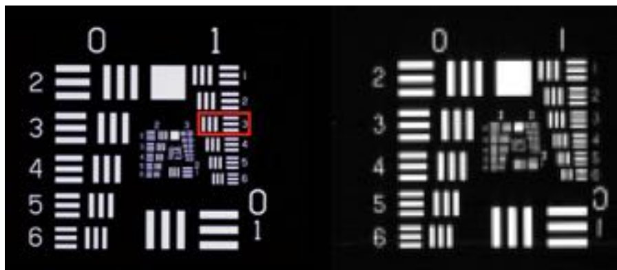
Fig. 25: USAF mask 1951 reference image (left). The pattern G = 1 , E = 3 indicated by the red box corresponds to the VIHI theoretical frequency f_{Nyquist} = 2.52 lines/mm. VIHI image of the mask (right) at wavelength \lambda = 590 nm. The VIHI slit (sample direction) is oriented towards the vertical axis and the image is acquired in time by scanning at one IFoV step along the horizontal axis. From Filacchione et al. (2017) .
