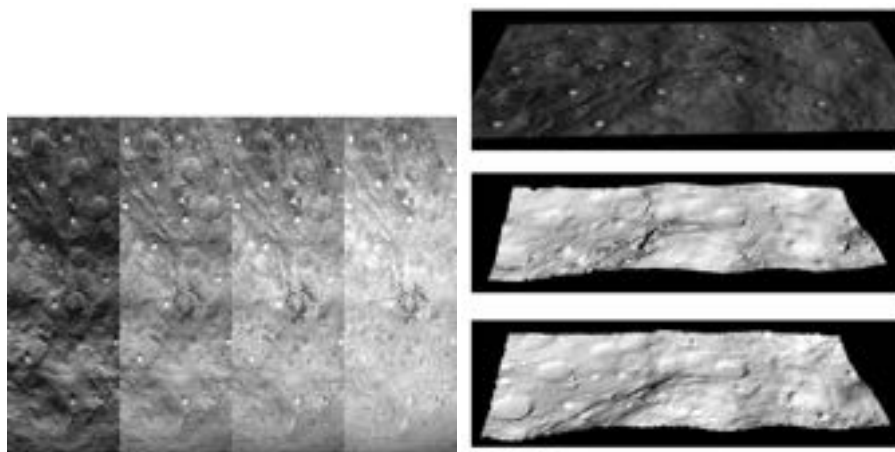
Fig. 22: The effect of four different illumination conditions for the anorthosite sample (left), with incidence angles of 10^\circ , 30^\circ , 50^\circ , and 70^\circ from left to right. The image obtained by one STC channel of the anorthosite target (top right), the photogrammetric DTM (middle right), and the DTM generated by the laser scanner (bottom right).
