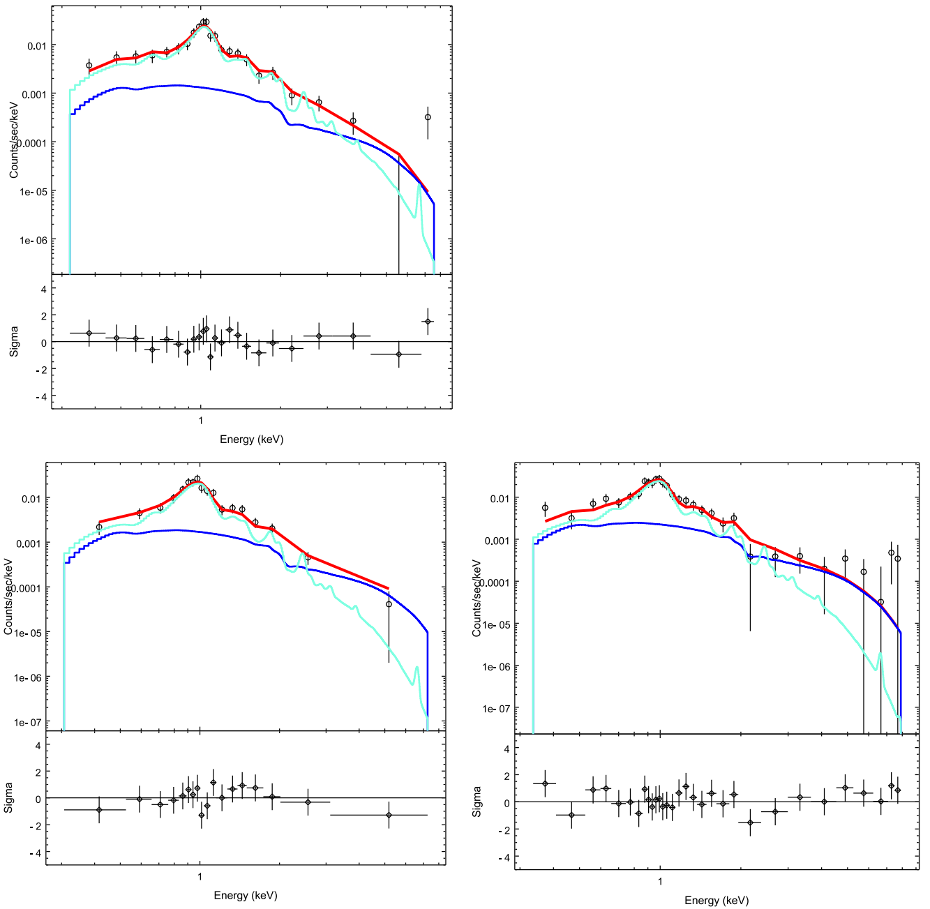
Figure 5. Comparison of spectral fitting results from three radial bins. (a) 1.34 ( -0.04 , +0.06 ) keV gas from the possible shock, the third bin in Figure 4, (b) 1.07 ( -0.03 , +0.09 ) keV gas from the inner region, the second bin in Figure 4, and (c) 1.08 ( -0.03 , +0.08 ) keV gas from the outer region, the fifth bin in Figure 4. The gas component is in cyan, the hard component (likely from the undetected LMXBs) in blue and the sum in red. In all three cases, the reduced \chi^2 is less than one.
