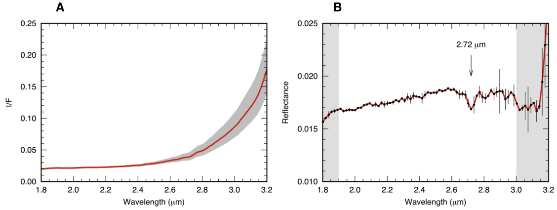
Fig. 1. NIRS3 near-infrared spectra of Ryugu. (A) Reflectance spectra including thermal emission. The range of variation in spectra acquired from the equatorial scan on July 10, 2018 are shown (gray) along with the average spectrum (red). I/F is the measured radiance divided by the solar flux. (B) An example of a thermally-corrected spectrum (observation date and time: 2018-07-10T06:02:22 UTC). Error bars are calculated based on the uncertainties in the element-to-element radiometric calibration (9). Shaded areas indicate regions with large calibration residuals. The absorption band indicated by the arrow at 2.72\ \mu\text{m} is due to OH.
