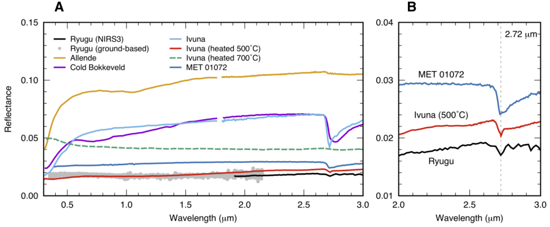
Fig. 3. Comparison of Ryugu with meteorite spectra. (A) The globally-averaged NIRS3 spectrum of Ryugu compared with laboratory spectra of meteorite samples: Ivuna (CI1), Cold Bokkeveld (CM2), MET 01072 (shocked CM2), and Allende (CV3). Details and references for the meteorite spectra are listed in Table S1. A ground-based visible and near-infrared spectrum of Ryugu (6) is also plotted. (B) Enlargement of (A) in the NIRS3 wavelength range.
