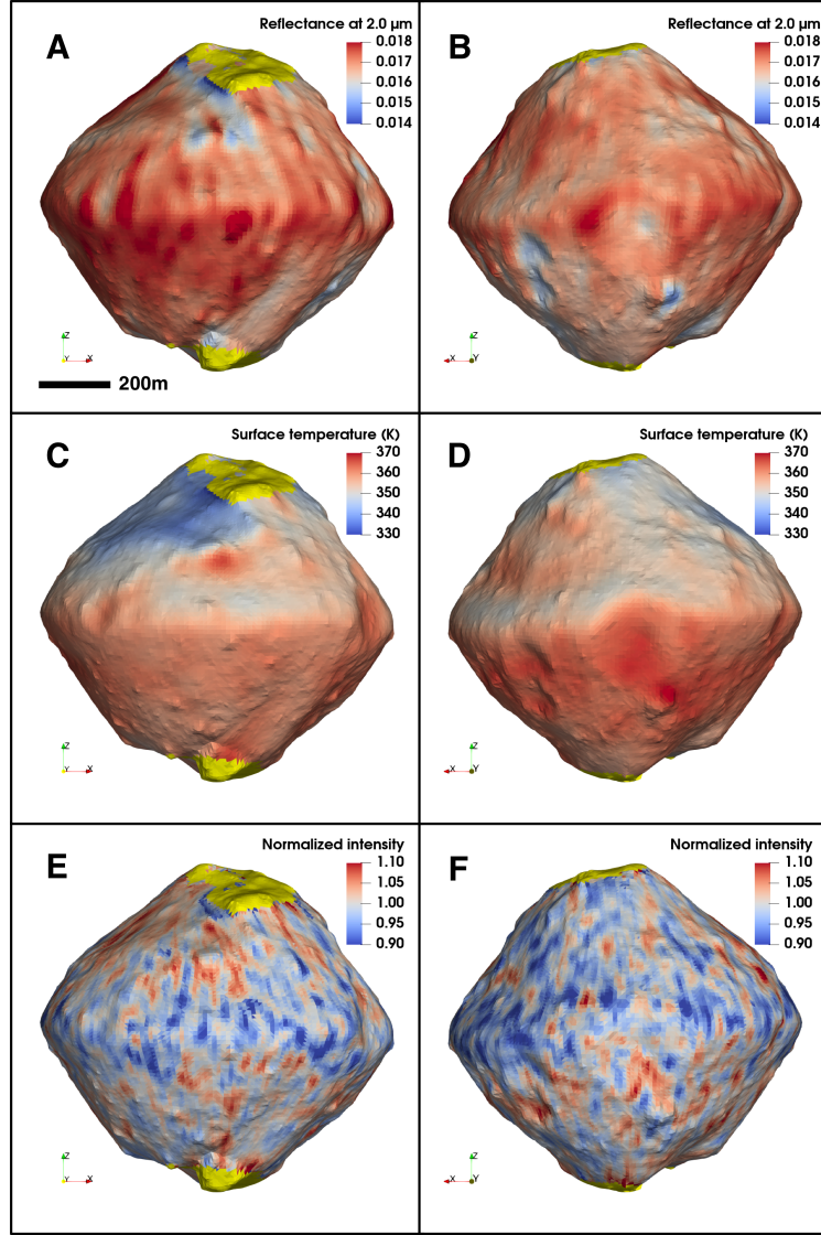
Fig. 2. NIRS3 spectral features projected onto the shape model of Ryugu (25). The left- and right-side views correspond to the western and eastern hemispheres, respectively. Yellow-shaded areas represent regions that were not observed. (A and B) Reflectance factor at 2.0 \mu\text{m} corrected to a standard viewing geometry (9). (C and D) Surface temperature (K) derived from the thermal emission component. (E and F) Normalized intensity of the 2.72 \mu\text{m} feature. The Z and X arrows indicate Ryugu's rotation axis and zero-longitude definition, respectively.
