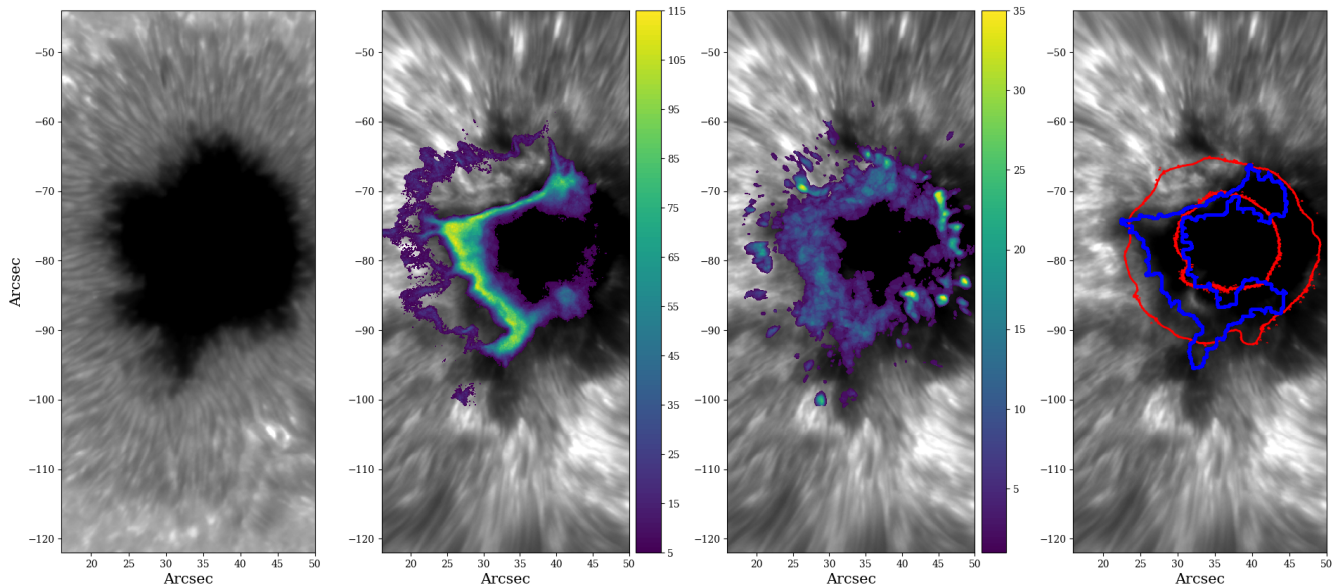
Figure 1. Left: IBIS Ca II red wing image of active region NOAA 12546, acquired at 8542.6 \text{ \AA} (line core +0.5 \text{ \AA} ). Middle-left: Ca II 8542 \text{ \AA} line core image, where the over-plotted colored pixels represent the locations where reversals in either Stokes Q/I_c , U/I_c or V/I_c spectropolarimetric profiles are detected between neighboring frames. The color scale indicates the total number of polarimetric reversals occurring in that pixel throughout the duration of the time series. Middle-right: Locations and occurrences of pixels that exhibit a change in their Stokes I/I_c magnitude exceeding 3\sigma above their quiescent value. Right: The red lines represent plasma- \beta = 1 isocontours spanning optical depths of ( \sim 450 \text{ km} ) -3 > \log_{10} \tau > -4 ( \sim 625 \text{ km} ). The blue contour represents an outer boundary that encompasses all locations that are deemed ‘active’ pixels (see Section 3.1).
