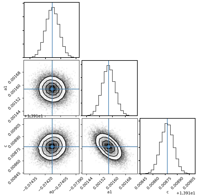
Figure 4. Modeling the imperfect temperature compensation of the spacecraft clock. Confidence intervals for the parameters of Equation (9), plotted using the corner library (Foreman-Mackey 2016).
