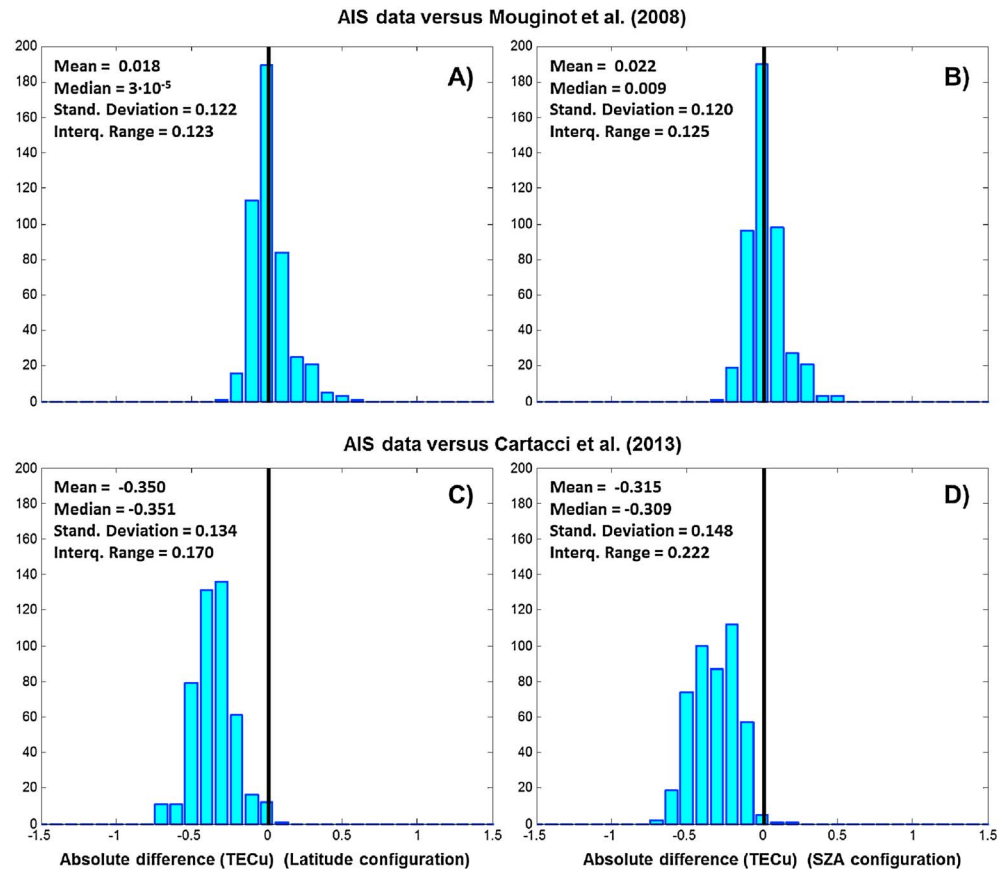
Figure 6. Absolute differences between the topside AIS-derived TEC and the TEC retrieved from the MARSIS subsurface mode: (a and b) Mouginito et al.'s method and (c and d) Cartacci et al.'s method. The total number of data points is 458 (19 orbits). (Figures 6a and 6c) Histograms of the absolute differences in TECu for the latitude as the varying parameter. (Figures 6b and 6d) Histograms of the absolute differences in TECu for the solar zenith angle as the varying parameter. The vertical black line marks the zero difference. The analysis confirms that the absolute differences between ionospheric data from AIS mode (topside ionosphere) and Mouginito et al.'s subsurface data (full ionosphere) are practically nonexistent, being a clear inconsistency (Figures 6a and 6b). The absolute differences between ionospheric data from AIS mode and Cartacci et al.'s subsurface data are higher (Figures 6c and 6d). It seems more realistic, although it is known that this latest subsurface retrieval overestimates the dayside TEC.
