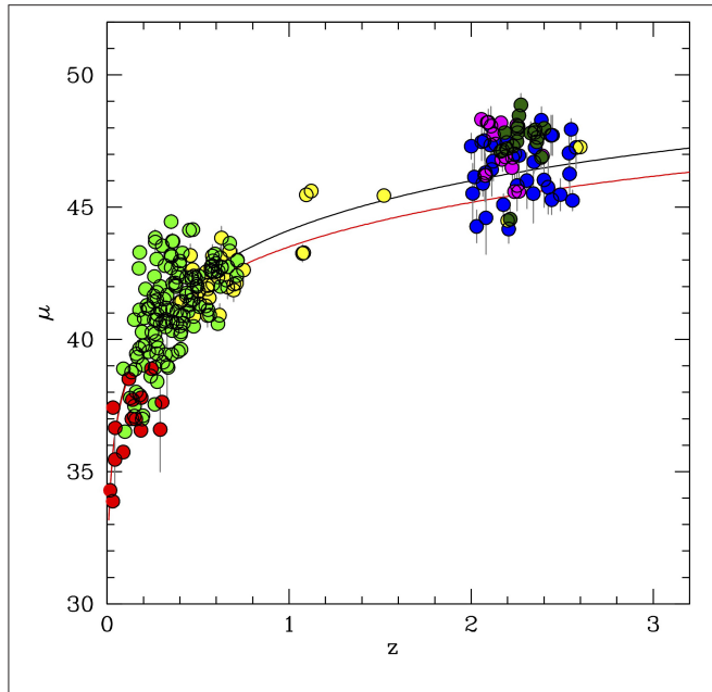
FIGURE 3 | Hubble diagram (distance modulus \mu vs. redshift z ) for several samples of xA quasars using virial luminosity distances from the FWHM of H \beta and AlIII \lambda 1860. Data points are color-coded according to sample and line employed: blue (●): Marziani and Sulentic (2014a) AlIII \lambda 1860; yellow (●): Marziani and Sulentic (2014a) H \beta ; green (●): Negrete et al. (2018) H \beta ; red (●): Du et al. (2016) H \beta ; dark green (●): Sniegowska et al., in preparation; magenta (●): Martínez-Aldama et al. (2018). The continuous lines trace the prediction for concordance \Lambda CDM (black) the Einstein-de Sitter (red) cosmology.
