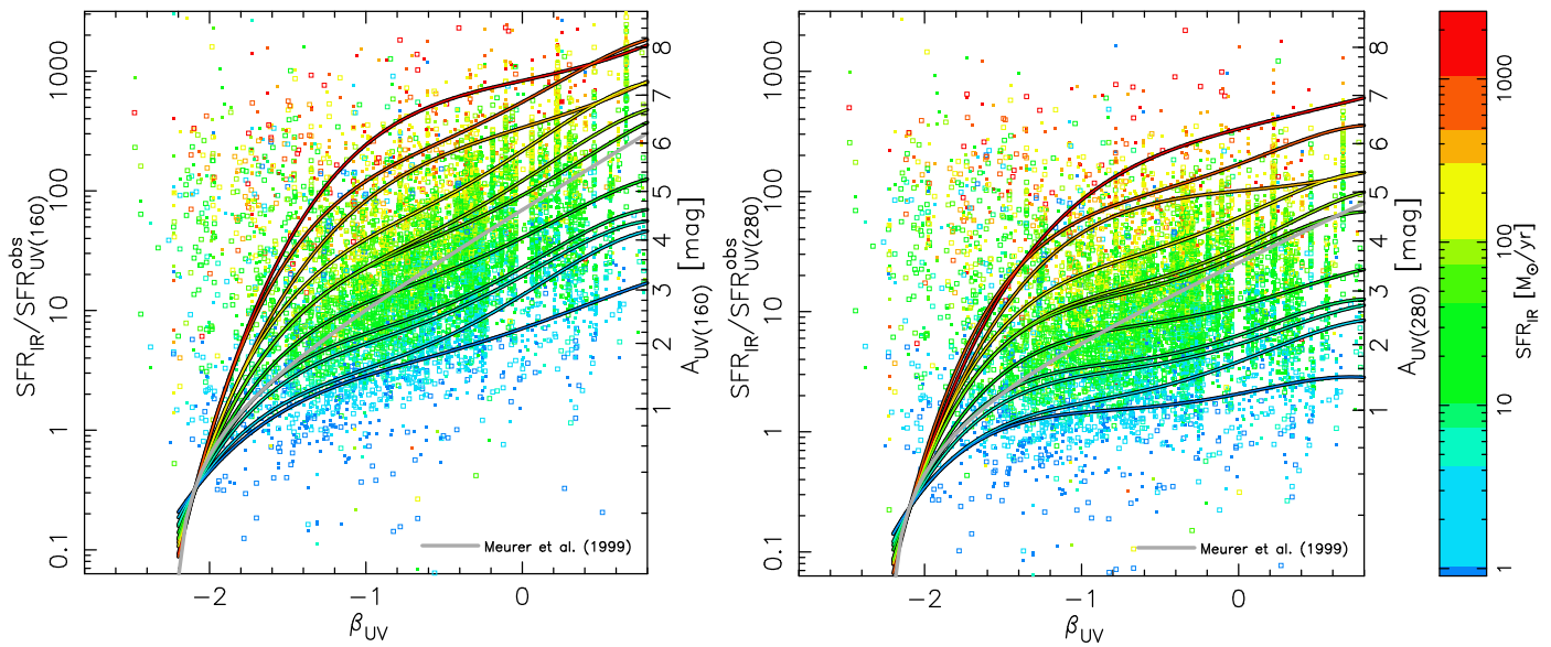
Figure 26. IRX- \beta_{UV} plots for the galaxies detected by MIPS/PACS/SPIRE in the five CANDELS fields. On the left, we show the results for UV-based SFR estimations based on the emission at 160 nm rest frame (Equation (D.4), Kennicutt 1998), and on the right for 280 nm (Equation (D.5), Bell et al. 2003). Galaxies with Herschel detections are plotted with filled symbols (and SFR_{IR} = SFR_{IR}^{obs} , see text for details); galaxies with just a MIPS detection are plotted with open symbols (and SFR_{IR} = SFR_{IR}^{W1} ). Colors represent different bins of IR-based SFR [or L(8-1000) ] as shown in the scale plotted on the right. The data for each bin has been fitted to a Chebyshev polynomial of order 5, shown with lines of the same color. The Meurer et al. (1999) relationship is plotted in gray (using the Calzetti et al. 2000 attenuation law to transform from far-UV to near-UV A_{UV} values). The IRX scale (on the left of each panel) is transformed into an attenuation scale (on the right of each panel) using Equation (4).
