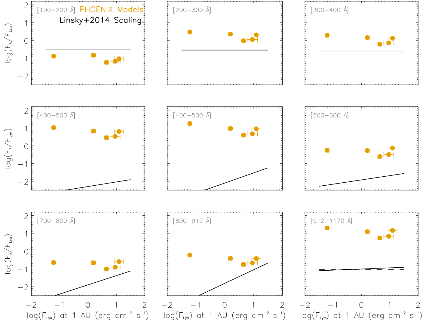
Figure B1. Estimated F_{\lambda}/F_{\text{Ly}\alpha} using the Linsky et al. (2014) scaling relationships (black) compared to the ratios of integrated fluxes in 100 Å wavelength bands to the Lyα flux computed from the median 0.4 \pm 0.05 M_{\odot} models (orange). The scaling relationships for wavelengths <400 Å are determined from EUVE observations of M stars. The relationship for 912–1170 Å is determined from FUSE observations of K5–M5 stars. The relationships for wavelengths between 400 and 912 Å are computed from solar models from Fontenla (2013).
