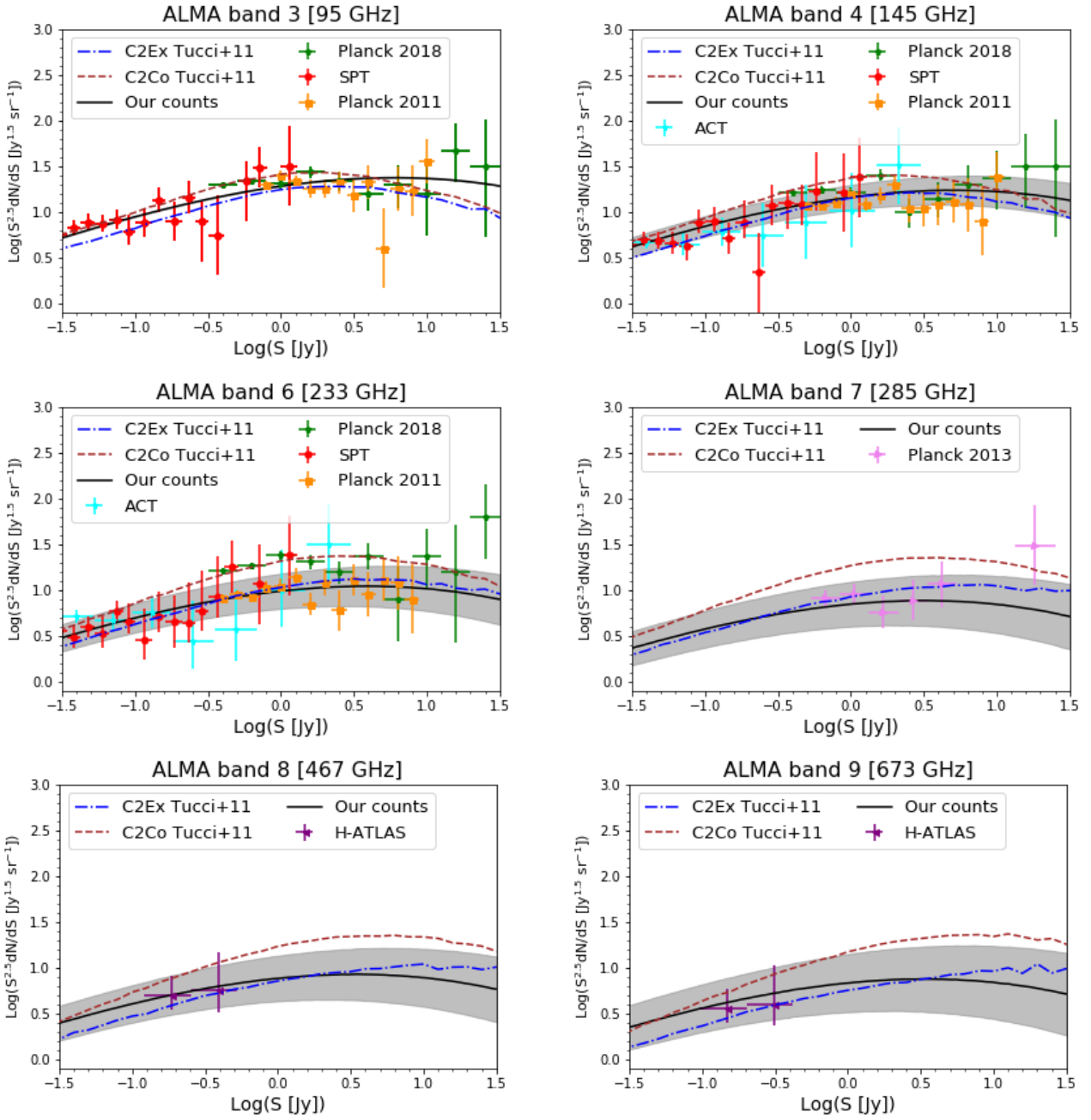
Figure 4. Euclidean normalized differential source counts of radio sources in the ALMA bands for which measurements for a substantial number of calibrators are available. The data are from Marsden et al. (2014, ACT), Mocanu et al. (2013, SPT), Planck Collaboration et al. (2011), Planck Collaboration et al. (2013) and Planck Collaboration Int. LIV (2018). The band 8 and band 9 data points are our own estimates using Table 1 of Negrello et al. (2017); the extrapolations of the 600 GHz (500 \mu m) flux densities given there to the effective frequencies of these 2 bands were done assuming S \propto \nu^{-0.62} , i.e. using the mean spectral index between Bands 8 and 9. The mean spectral index between Bands 6 and 8 ( -0.45 ) was used to convert the Planck Collaboration et al. (2013) counts from 353 to 285 GHz. The dot-dashed blue line and the dashed brown line show two models by Tucci et al. (2011).
