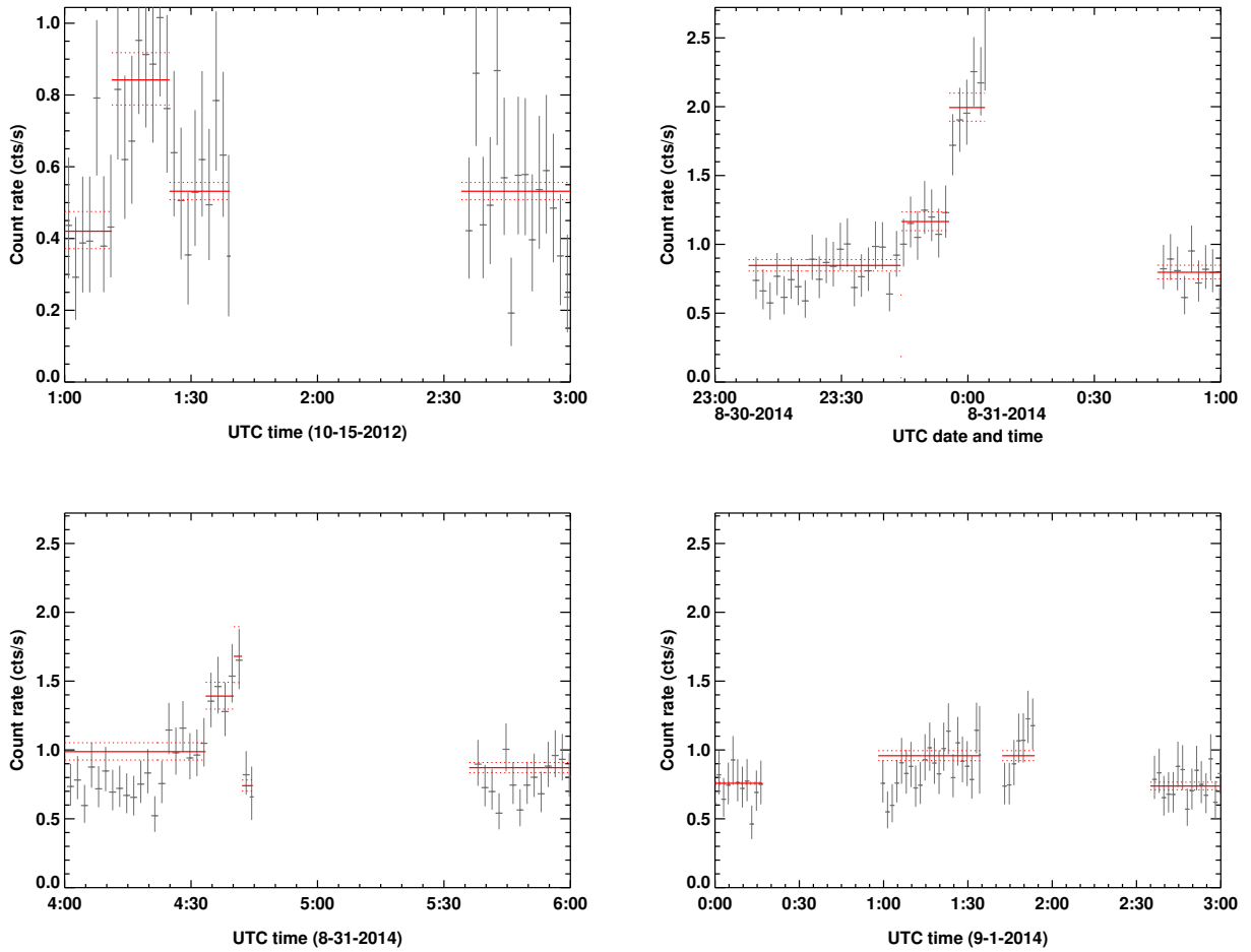
Figure 1. NuSTAR 3 – 79 keV light curves showing previously unreported flares with > 3\sigma detections, including flare Nu5 (upper left), Nu7 (upper right), Nu8 (lower left) and Nu9 (lower right). The NuSTAR light curves are deadtime, PSF, and vignetting corrected and extracted from a 30'' radius circle centered on Sgr A* in 100s bin. The light curves of the four bright flares Nu1, Nu2, Nu3 and Nu6 are shown in Figure 1 and 2 in Barrière et al. (2014). Flares Nu4 and Nu10 are not significantly detected with NuSTAR data only. The Nu4 Chandra light curve is presented in Neilsen et al. (2013); the Nu10 XMM-Newton light curve is presented in Ponti et al. (2015).
