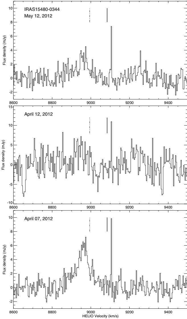
Fig. 2. \text{H}_2\text{O} maser spectra observed towards IRAS 15480-0344 with the GBT on April 7 ( bottom panel ), April 12 ( middle panel ), and May 12, 2012 ( top panel ). Channel spacing is 3.3 \text{ km s}^{-1} . The vertical line indicates the recession velocity of the galaxy. The dash-dotted line marks the velocity of the maser spot M2, detected with the VLBA (Sect. 4.2). The velocity scale is with respect to the heliocentric frame and uses the optical convention.
