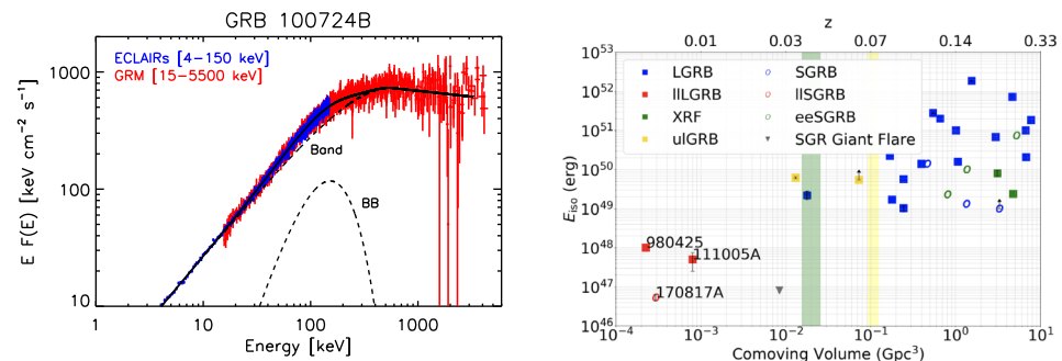
Figure 3. Left panel: The multi-component (band plus blackbody) prompt emission spectrum of the Fermi/GBM detected GRB 100724B, simulated as it would have been seen by ECLAIRS and GRM. The two instruments together will be capable to well characterize the peak energy and all the features of the prompt emission of GRBs. Adapted with permission from ref. [2], Copyright Year: 2017, Copyright Owner: Springer. Right panel: ECLAIRS on-axis count Signal-to-Noise ratio (SNR) for short high-energy transients in the local Universe: Long and Short GRBs (LGRB, SGRB), X-ray Flashes (XRF), ultra-long GRBs (ulGRBs), and Soft Gamma-ray Repeater (SGR) giant flares. The orange horizontal band represents the detection threshold of ECLAIRS at SNR = 6.5. The green and yellow bands represent the O4 LIGO distance sensitivity limits for double neutron stars and neutron star-black hole mergers, respectively. The light grey trails represent the evolution of the on-axis count SNR with the redshift. Adapted with permission from ref. [4], Copyright Year: 2020 Copyright Owner: Springer.
