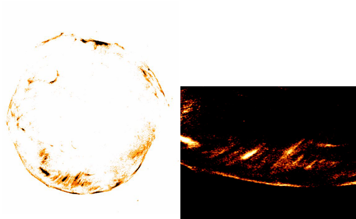
Figure 3. Left: Chandra X-ray image of Tycho's SNR in 4-6 keV photon energy regime. Right: Zoomed X-ray stripes in 4-6 keV Chandra image of Tycho's SNR discovered by [11].
