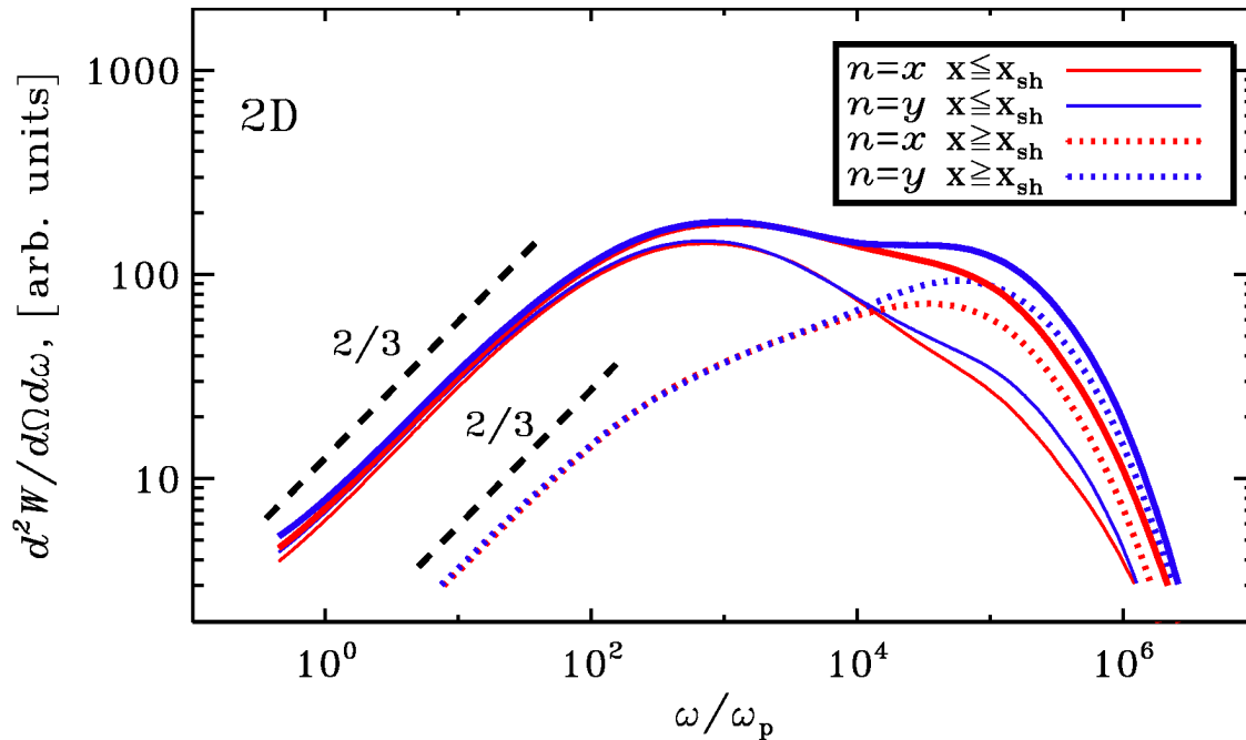
Figure 12. Ab initio photon spectrum (thick solid lines) from the 2D PIC simulation of an unmagnetized (i.e., \sigma = 0 ) shock [362]. Red lines are for head-on emission (along the shock direction of propagation), blue lines for edge-on emission (along the shock front). The slope at low frequencies is 2/3 (black long-dashed lines), proving that the spectra are consistent with synchrotron radiation from a 2D particle distribution (in 3D, the predicted slope of 1/3 is obtained). By separating the relative contribution of post-shock (thin solid lines) and pre-shock (dotted lines) particles, one sees that pre-shock particles contribute significantly to the total emission (thick solid lines), especially at high frequencies. Frequencies are in units of the plasma frequency \omega_p .
