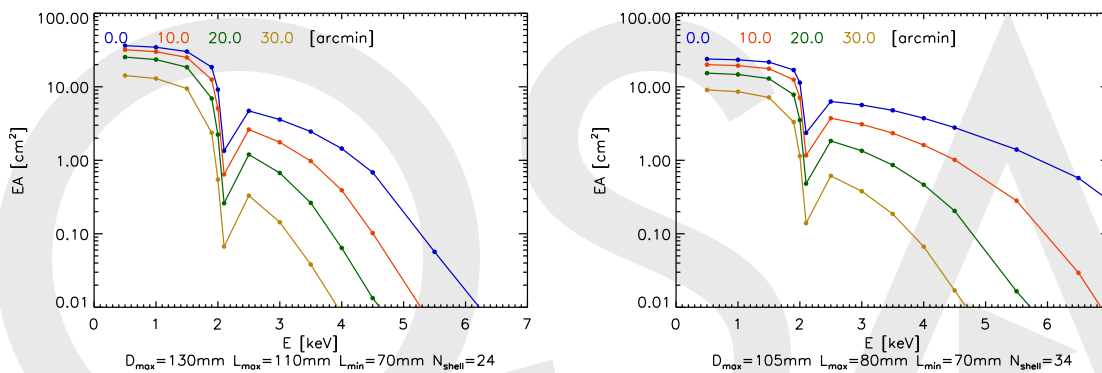
Fig. 8. Effective area (EA) as a function of energy for various off-axis locations (on-axis: blue; 10': orange; 20': green; 30': yellow) for the large ( left ) and small ( right ) designs. This is a different projection of the information present in Figure 7.
