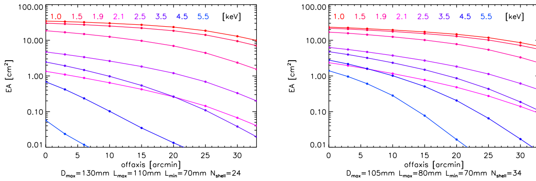
Fig. 7. Effective area (EA) as a function of off-axis location for the large ( left ) and small ( right ) designs. The different colored curves are for different photon energies, as in Figure 5. A different projection of the same information, EA vs. energy for different off-axis angles is shown in Figure 8.
