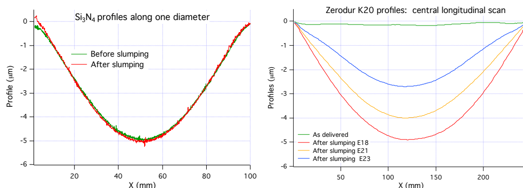
Fig. 9. Shape stability of \text{Si}_3\text{N}_4 compared to the deformation of the Zerodur K20: on the left, the \text{Si}_3\text{N}_4 profiles along one diameter, as measured with the Zeiss contact profilometer before and after the slumping; on the right, the K20 profiles along the central longitudinal scan, as measured with the LTP after several slumping cycles.
