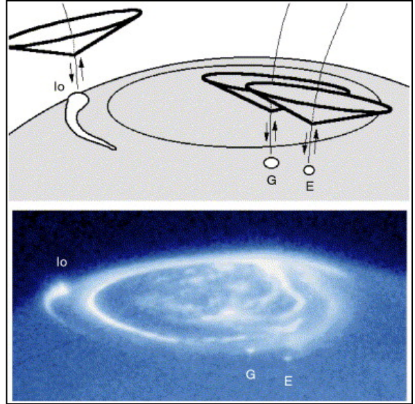
Fig 2. (Bottom) HST UV image of northern Jovian auroral regions, showing clearly the bright main auroral oval and the footprints of Io (plus a tail-like structure), Ganymede and Europa flux tubes. Courtesy: R. Prangé , L. Pallier, and J.T. Clarke. (Top) Sketch of radio emission hollow conical beams produced above the UV hot spots by the energetic electrons precipitated along the satellite flux tubes or reflected upwards by magnetic mirroring. [Zarka et al., 2007]
