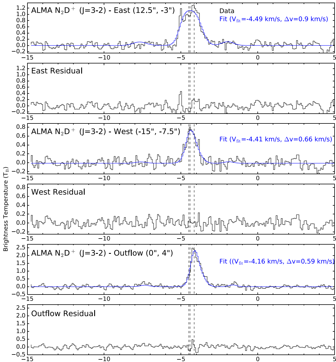
Figure 24. ALMA N_2D^+ spectra taken toward three positions, showing the spectrum and hyperfine fit in one panel and the residual of the fit below. The coordinates denoted for east, west, and outflow are relative to the position of IRS1 in Figure 16, and the extraction regions are also drawn as circles in the upper right panel of that Figure. The east spectrum has the highest residual, which is likely due to the two velocity components that are apparent in Figure 17. The two blended components in the east spectrum cause the broader line width in the fit. The west position is dominated by a single-velocity component, and the outflow position has a low residual.
