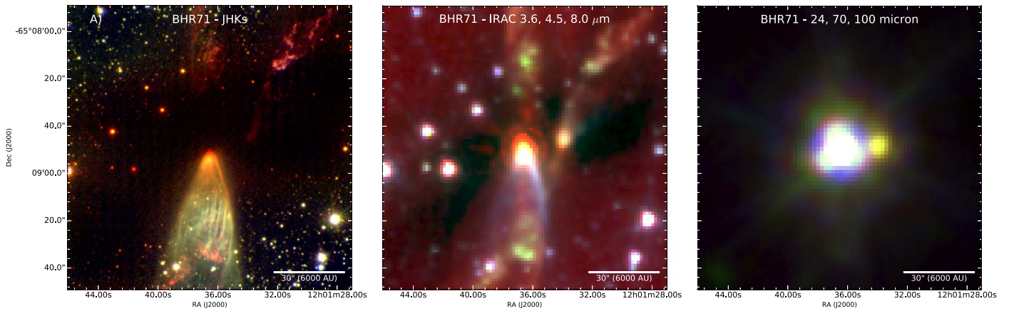
Figure 1. False-color images of BHR71 at multiple wavelengths. The left panel shows BHR71 as viewed in the near-infrared in Ks (PANIC), H (PANIC), and J bands (ISPI). The outflow cavity from the blueshifted outflow of IRS1 is quite prominent and the outflow cavity from IRS2 is not distinct, but several knots are apparent in the northwest portion of the image. The middle panel shows the Spitzer 3.6, 4.5, and 8.0 \mu\text{m} images on the same scale. IRS1 is still dominant, but IRS2 is much more apparent. The right panel shows the Spitzer 24 \mu\text{m} image along with Herschel 70 and 100 \mu\text{m} imaging that clearly resolves the mid- and far-infrared emission that is directly associated with both IRS1 and IRS2. IRS1 is quite prominent at all three wavelengths, but IRS2 is not strongly detected until 70 and 100 \mu\text{m} because of its deeply embedded nature. All images map the longest wavelength to red, the intermediate wavelength to green, and the shortest wavelength to blue.
