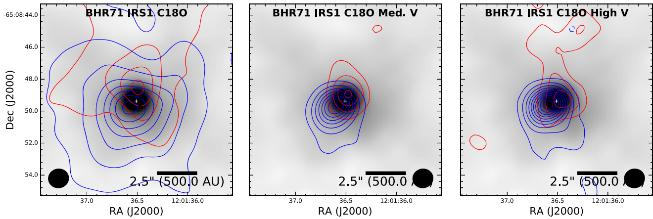
Figure 19. C^{18}O red- and blueshifted integrated intensity maps toward IRS1 (using 12m+ACA+TP data) shown in different velocity ranges and overlaid on the 1.3 mm continuum image. The low-velocity C^{18}O clearly is influenced by the outflow, but at moderate and higher velocities, the C^{18}O begins to trace a velocity gradient orthogonal to the outflow, the expected velocity gradient direction for rotation. The low-velocity emission is integrated between -5.8 to -4.4 \text{km s}^{-1} and -4.4 to -3.2 \text{km s}^{-1} , and \sigma_{\text{red,blue}} = 0.09, 0.1 \text{K km s}^{-1} , and the contours are drawn starting at 30\sigma and increase in intervals of 30\sigma . The moderate-velocity emission is integrated between -6.2 to -5.6 \text{km s}^{-1} and -3.6 to -2.8 \text{km s}^{-1} , and \sigma_{\text{red,blue}} = 0.08, 0.07 \text{K km s}^{-1} , and the contours are drawn starting at 10\sigma and increase in intervals of 10\sigma . The high-velocity emission is integrated between -6.3 to -5.8 \text{km s}^{-1} and -3.0 to -2.5 \text{km s}^{-1} , and \sigma_{\text{red,blue}} = 0.06, 0.06 \text{K km s}^{-1} , and the contours are drawn starting at 3\sigma ( 5\sigma ) and increase in intervals of 3\sigma ( 5\sigma ); the values in parentheses correspond to the blue contours. The 12m+ACA+TP data were used to generate this figure.
