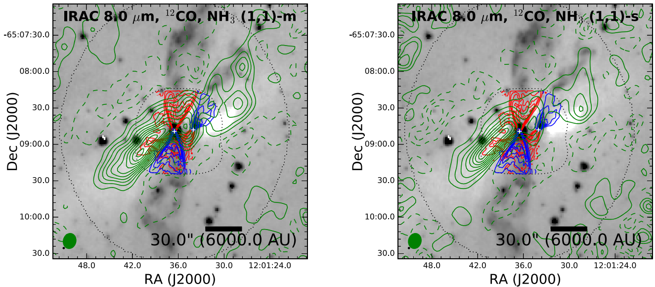
Figure 9. Integrated intensity contours from the ATCA \text{NH}_3 (1, 1) observations (green) overlaid on the Spitzer 8 \mu\text{m} image (inverse grayscale). The integrated intensity of the main \text{NH}_3 lines is shown in the left panel and the satellite lines are presented in the right panel (between -12.6 to -11.4 \text{km s}^{-1} ). We also overlay the ^{12}\text{CO} red- and blueshifted integrated intensity contours (with corresponding colors) from Figure 6, showing the relationship of the outflow with the dense gas. The \text{NH}_3 (1, 1) emission at this higher resolution shows excellent correspondence with the 8 \mu\text{m} absorption feature of the envelope on the background, and the \text{NH}_3 maps exhibit a cavity and depressions toward the location of IRS1. IRS2 is located directly beside an \text{NH}_3 peak. The \text{NH}_3 main and (satellite) contours start at 5\sigma ( 3\sigma ) and increase in 5\sigma ( 3\sigma ) intervals, where \sigma = 0.075 \text{K km s}^{-1} ( 0.072 \text{K km s}^{-1} ). A -5\sigma ( -3\sigma ) contour is also drawn.
