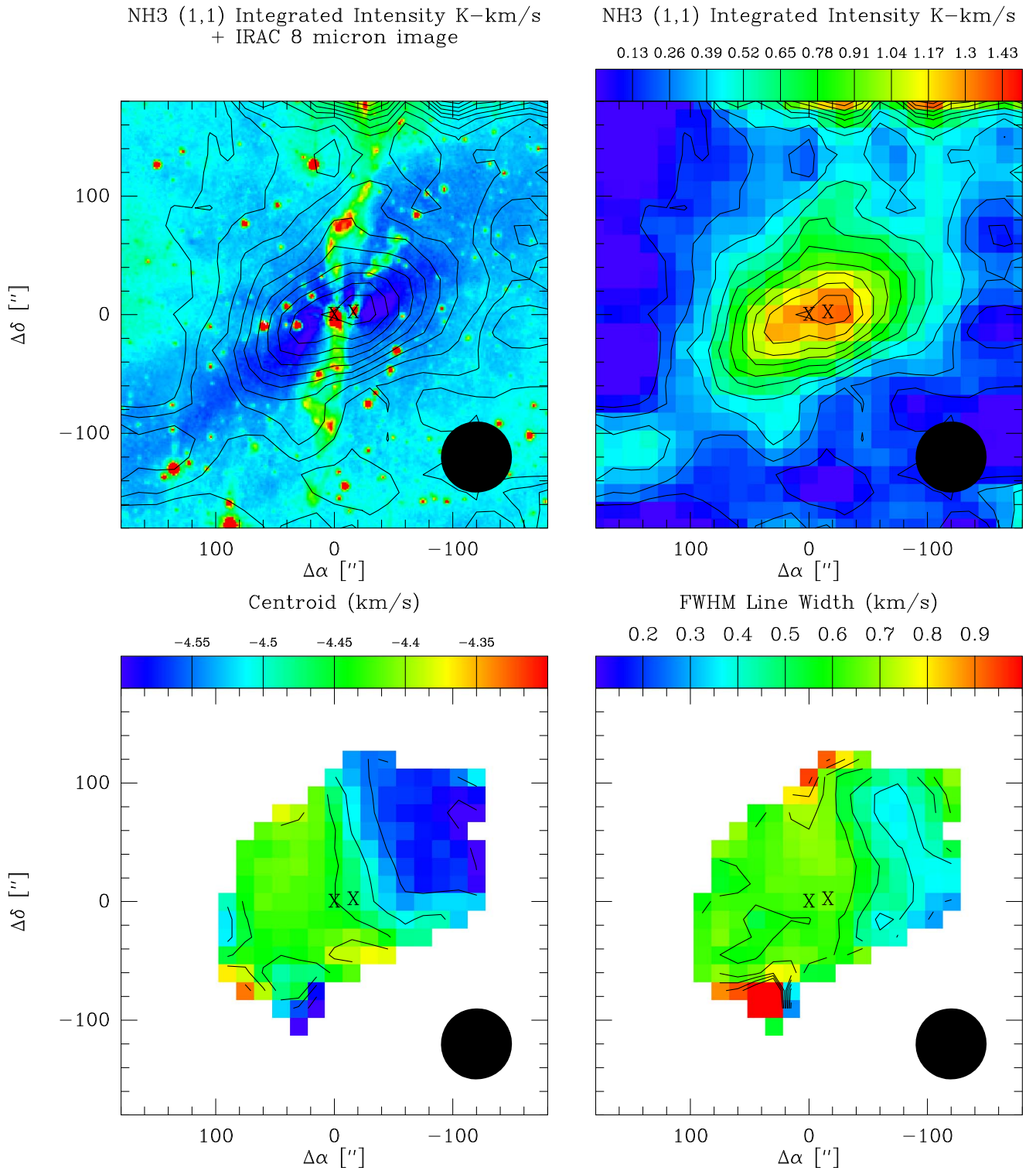
Figure 8. Parkes single-dish NH 3 (1, 1) maps. The upper left panel shows the integrated intensity of the main NH 3 (1, 1) hyperfine lines overlaid on the Spitzer 8 \mu m image (color scale). The upper right panel shows just the integrated intensity of the main NH 3 (1, 1) hyperfine lines (color scale and contours). The lower left panel shows the line-center velocity derived from a fit to all the NH 3 (1, 1) hyperfine lines, and the lower right panel shows the line width also derived from fitting all hyperfine components. The integrated intensity peaks toward the position of IRS2, and the velocity map shows a very small gradient across the source, only about a 0.15 \text{ km s}^{-1} differential. The line-width map shows that the lines are narrow, at most only about 0.6 \text{ km s}^{-1} wide. The positions of the IRS1 and IRS2 are marked with crosses. The intensity levels in the top panels are from the integrated intensity map of the main hyperfine lines between -6.5 to -2.2 \text{ km s}^{-1} ; the intensity levels start at and increase in 3\sigma intervals, where \sigma = 0.045 \text{ K km s}^{-1} .
