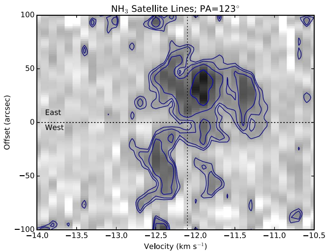
Figure 13. Position–velocity diagrams of \text{NH}_3 taken in a 10'' wide strip along a position angle of 123^\circ east of north, centered on IRS1. The extracted region is bounded by the dashed lines in the upper right panel of Figure 10. The top panel shows the PV diagram of the main \text{NH}_3 hyperfine lines, and the bottom panel shows a PV diagram of a set of \text{NH}_3 satellite hyperfine lines that are not as closely spaced as the main lines.
