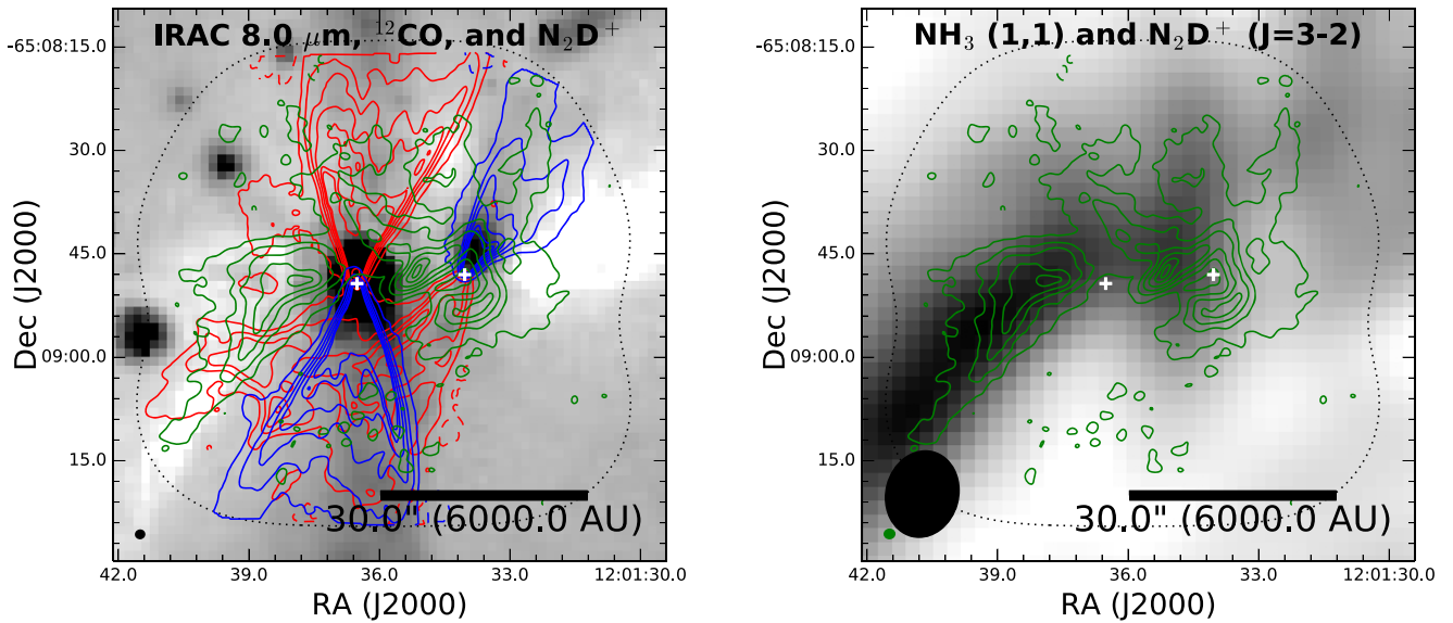
Figure 15. Integrated intensity contours from the ALMA N_2D^+ ( J = 3 \rightarrow 2 ) observations overlaid (green) on the Spitzer 8.0 \mu\text{m} image (inverse grayscale) in the left panel and N_2D^+ is overlaid (green) on the ATCA NH_3 (1, 1) integrated intensity map (inverse grayscale) in the right panel. We also overlaid the ^{12}CO blue- and redshifted integrated intensity contours (with corresponding colors) from Figure 6. The extent of C^{18}O shown in Figure 6 is consistent with the size of the N_2D^+ deficit regions. There is some correspondence on the east side of the N_2D^+ and the 8 \mu\text{m} absorption of the envelope, but less than the ATCA NH_3 due to the smaller area mapped by ALMA. The ALMA N_2D^+ corresponds well with the NH_3 on the eastern side of the map, and the emission toward IRS1 is lower in both NH_3 and N_2D^+ . Near IRS2, the correspondence of N_2D^+ and NH_3 is not as close: the peak of NH_3 east of IRS2 corresponds with the N_2D^+ peak, but N_2D^+ east and south of IRS2 has lower NH_3 intensity. The N_2D^+ contours start at 5\sigma and increase in 10\sigma intervals, where \sigma = 0.098 \text{ K km s}^{-1} .
