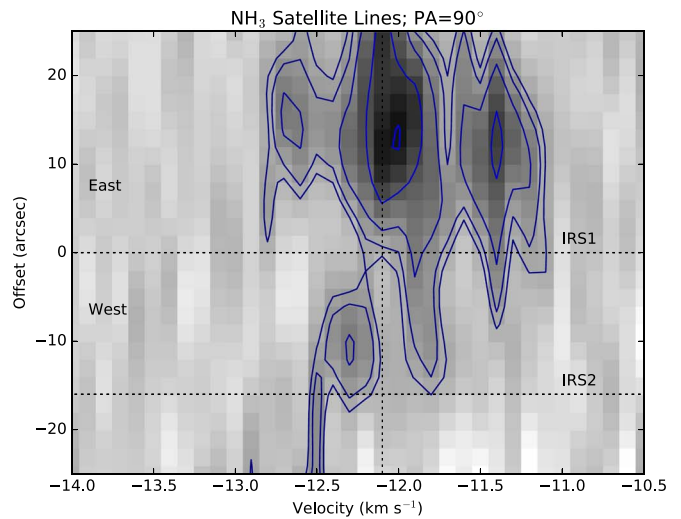
Figure 14. Position–velocity diagrams of \text{NH}_3 taken in a 10'' wide strip in the east–west direction, centered on IRS1. The region extracted is bounded by the dashed lines in the upper right panel of Figure 11. The top panel shows the PV diagram of the main \text{NH}_3 hyperfine lines, and the bottom panel shows a PV diagram of a set of \text{NH}_3 satellite hyperfine lines that are not as closely spaced as the main lines.
