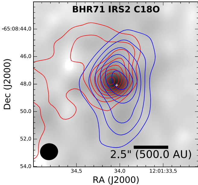
Figure 20. C^{18}O red- and blueshifted integrated intensity maps toward IRS2 (using 12m+ACA+TP data). A velocity gradient is evident, in a direction that is nearly orthogonal to the outflow. However, the velocity gradient direction is in the opposite sense with respect to the gradient direction in IRS1. The C^{18}O emission is integrated between -5.1 to -4.4 \text{km s}^{-1} and -4.4 to -3.5 \text{km s}^{-1} , and \sigma_{\text{red,blue}} = 0.08, 0.074 \text{K km s}^{-1} . The red and (blue) contours are drawn starting at 15\sigma ( 35.0\sigma ) and increase in intervals of 5\sigma ( 10\sigma ).
