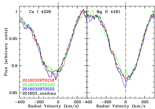
Fig. 3. Ca I 4226 Å and Mg II 4481 Å lines observed with FEROS during the night of 2016-03-28/29. The spectra have been rebinned to a pixel spectral resolution of 6.39 km s ^{-1} . The date and UT of each spectrum are indicated. Black dashed line: median of the four-day period shown for comparison. We note the different behaviour of the extra absorption features of each line when compared to their median spectra. The vertical dashed line corresponds to a radial velocity of 3 km s ^{-1} (see text in Sect. 4.2 and Fig. 5).
