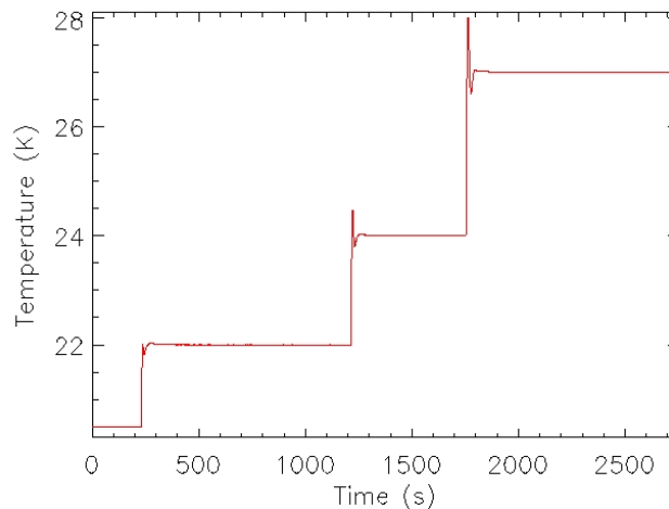
Figure -8: FEM temperature step during the RCA_THF test
