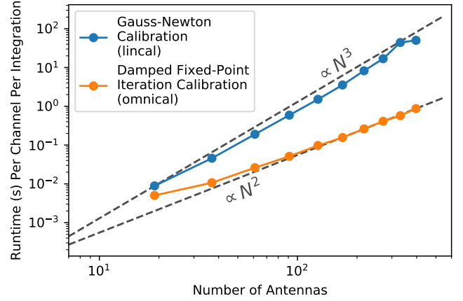
Figure 2. omnical, the damped fixed-point iteration algorithm we describe in Section 2.2.3 that avoids matrix inversion converges much faster than the lincal while achieving the same level of precision. Here we show the per-frequency and per-integration runtime for the two algorithms using single-precision floating point variables. The simulation uses increasingly large hexagonal arrays and simulates redundant visibilities using the same technique as the one described in Figure 1 and Section 2.2.1.
