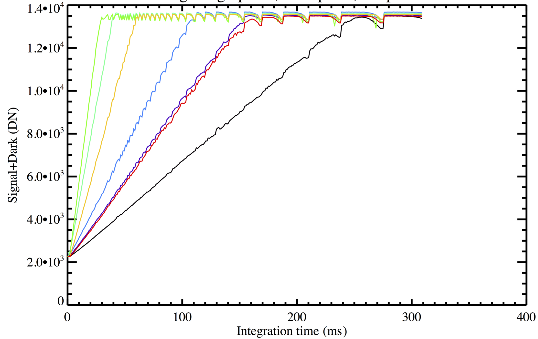
Integrating Sphere, 2 lamps on, sample=128
