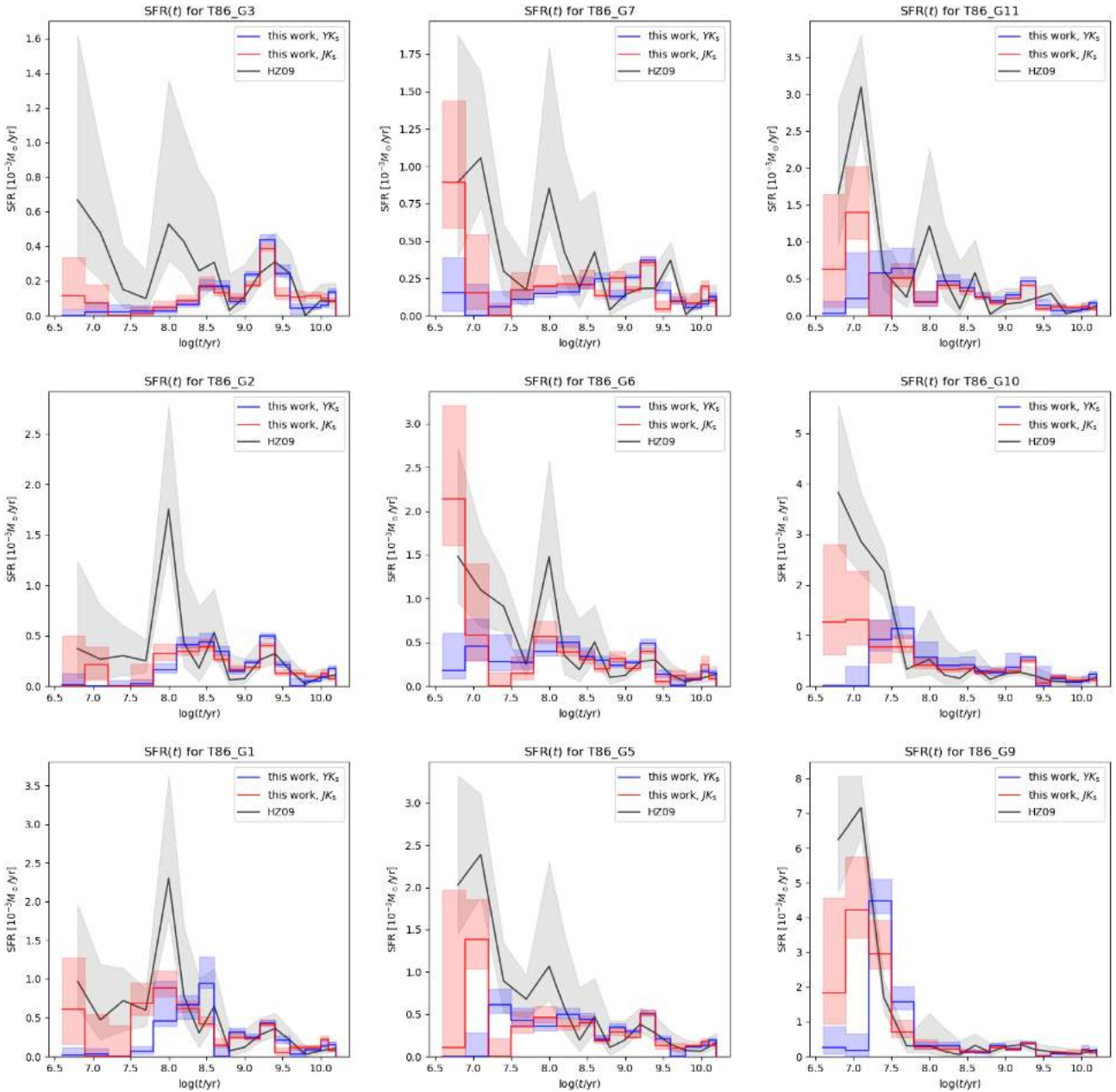
Figure 15. The same as Fig. 14 but for the southern section of the tile LMC 8.6, covering part of the star forming area known as Constellation III.
