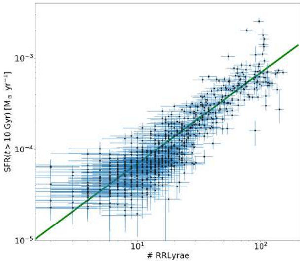
Figure 7. Comparison between the SFR(t) at very old ages, derived from JK_s data, with the number of RR Lyrae in each subregion. The error bars correspond to the 68 per cent confidence interval of the SFR, and to the square root of star counts. The green line presents the mean relation derived assuming a perfect proportionality between these quantities: its slope is of 1.45 \times 10^5 RR Lyrae per unit M_\odot \text{yr}^{-1} .
