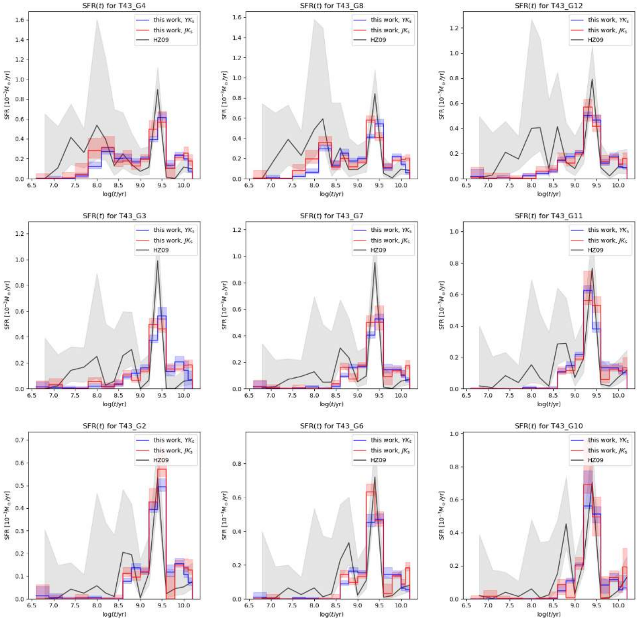
Figure 14. Comparison between our SFR(t) and those of Harris & Zaritsky (2009), for subregions covering the northern three-fourths of the tile LMC 4.3. They are plotted in the same way as they appear in the sky, with northernmost subregions at the top and westernmost subregions to the right. The different curves illustrate our derived SFR(t) , and the HZ09 SFR(t) resampled for the same area. The full lines correspond to the median values of the SFR(t) , while the shaded areas correspond to the 68 per cent confidence intervals.
