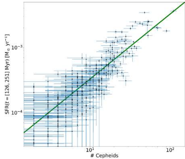
Figure 8. Comparison between the SFR(t) at ages between 126 and 251 Myr, derived from the JK_s data, with the number of Cepheids in each subregion. The error bars correspond to the 68 per cent confidence interval of the SFR, and to the square root of star counts. The green line presents the mean relation derived assuming a perfect proportionality between these quantities: its slope is of 3.07 \times 10^4 Cepheids per unit M_\odot \text{yr}^{-1} .
