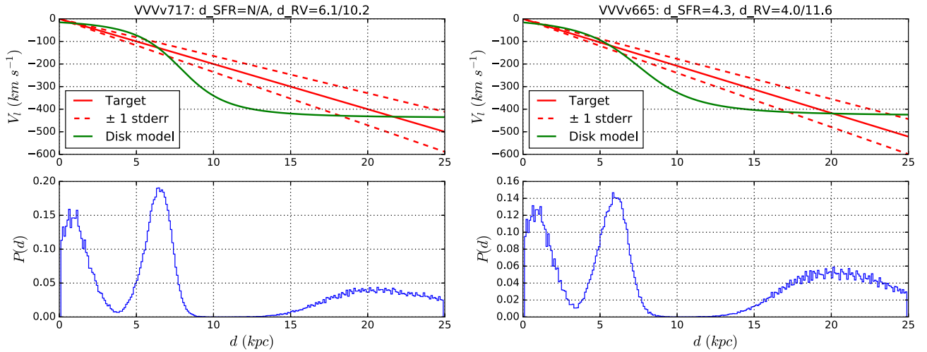
Figure 27. Upper left: our Galactic disc rotation model at l = 337^{\circ}68 , and projected tangential velocity of VVVv717 (Contreras Peña et al. 2017) using its VIRAC proper motion and uncertainty at the range of heliocentric distances covered by our disc model and a relative-to-absolute correction based on a Besançon synthetic stellar population. Upper right: the same but for VVVv665 at l = 331^{\circ}72 . Lower left: distance probability distribution of VVVv717 from intersection points between 100 000 Monte Carlo samples drawn from the VIRAC proper motion and uncertainty, and a peculiar motion of very young (blue) objects of 0 \pm 15 \text{ km s}^{-1} (Dehnen & Binney 1998, both normally distributed). Lower right: the same but for VVVv665. The Contreras Peña et al. (2017) distance estimates for the two sources were based on a similar method but using radial velocity instead of proper motion and also in the case of VVVv665 an estimate based on the distance to a star formation region relatively near to the target ( d_{\text{SFR}} ).
