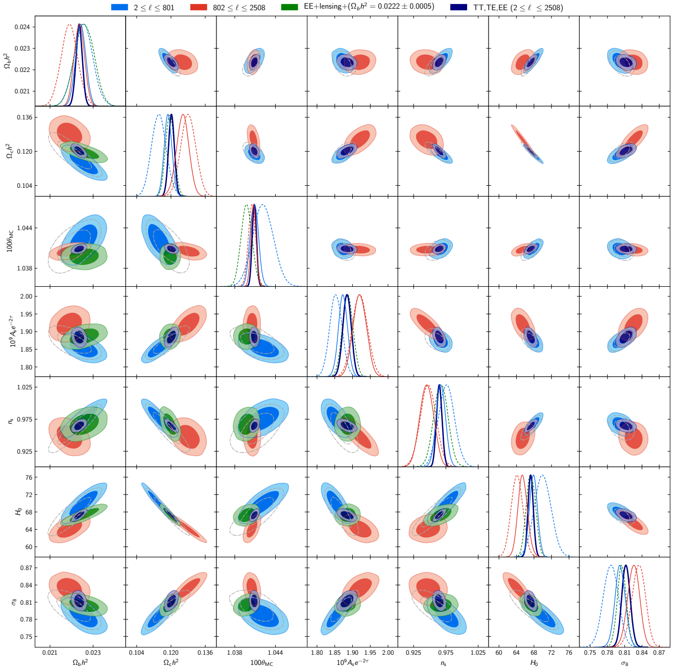
Fig. 21. Base- \Lambda CDM 68% and 95% parameter constraint and contours from the CMB power spectra using \ell \leq 801 (blue), compared to \ell \geq 802 (red). All results use the plik_lite Planck likelihood, and also include the low- \ell SimAll “lowE” likelihood to constrain the optical depth \tau ; the Commander likelihood is used for temperature multipoles \ell < 30 . The lower triangle contains the Planck temperature likelihoods, which show a moderate tension between high and low multipoles; however, they intersect in a region of parameter space consistent with the nearly-independent constraint from EE+lensing combined with a conservative prior \Omega_b h^2 = 0.0222 \pm 0.0005 , motivated by element-abundance observations (green). The upper triangle shows the equivalent results from Planck TT,TE,EE+lowE at low and high multipoles. The full combined result from Planck TT,TE,EE+lowE is shown as the navy contours. The unfilled grey contours show the result for multipoles 30 \leq \ell \leq 801 (that is, removing the low- \ell Commander likelihood that pulls parameters to give lower temperature power, due to the dip below \ell \approx 30 ). The diagonal plots are the marginalized parameter constraints, where results corresponding to the lower triangle are shown dashed, while the upper triangle are the solid curves.
