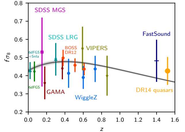
Fig. 14. Constraints on the growth rate of fluctuations from various redshift surveys in the base- \Lambda CDM model: dark cyan, 6dFGS and velocities from SNe Ia (Huterer et al. 2017); green, 6dFGS (Beutler et al. 2012); purple square, SDSS MGS (Howlett et al. 2015); cyan cross, SDSS LRG (Oka et al. 2014); dark red, GAMA (Blake et al. 2013); red, BOSS DR12 (Alam et al. 2017); blue, WiggleZ (Blake et al. 2012); olive, VIPERS (Pezzotta et al. 2017); dark blue, FastSound (Okumura et al. 2016); and orange, BOSS DR14 quasars (Zarrouk et al. 2018). Where measurements are reported in correlation with other variables, we here show the marginalized posterior means and errors. Grey bands show the 68% and 95% confidence ranges allowed by Planck TT,TE,EE+lowE+lensing.
