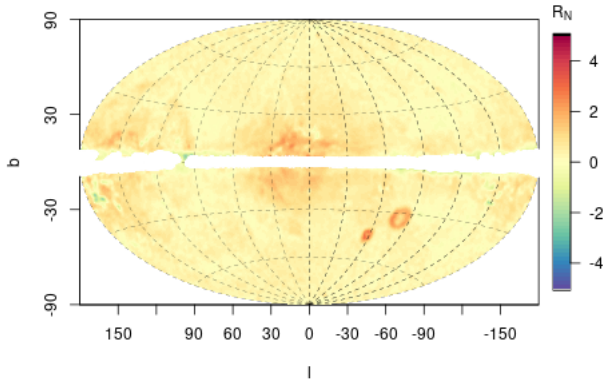
Fig. 31. Comparison of the total galactic extinction map (a0) with Planck E(B - V) normalised by the error R_N = (a_0 - E(B - V)) \times 3.1 / (a_0_{\text{uncertainty}} \times \sqrt{\text{num\_tracers\_used}}) . The white area corresponds to locations with \text{status} > 0 .
