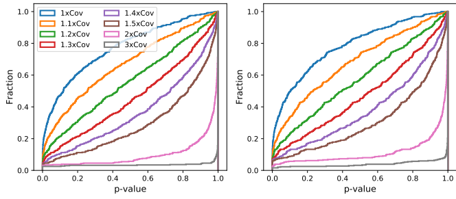
Fig. 25. Same as Fig. 24 for the 437 pairs that are fainter than G = 16 mag, but have a covariance matrix (Cov) of one to three times its original value for the two bands BP (left) and RP (right).
