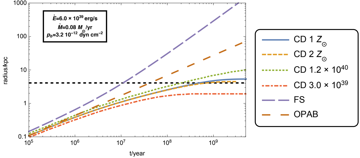
Fig. 4.— Radius of the bubble contact discontinuity (CD) and forward shock (FS) vs. time for \dot{E} = 6 \times 10^{39} erg/s and solar metallicity (unless otherwise marked) and \dot{M} = 0.08 M_{\odot}/\text{yr} (fixed); the atmosphere has pressure 2.0 \text{ eV cm}^{-3} \simeq 3.2 \times 10^{-12} \text{ dyn cm}^{-2} . Contact discontinuity (CD) curves are: i) solid blue for \dot{E} = 6.0 \times 10^{39} erg/s; ii) dashed orange for \dot{E} = 6.0 \times 10^{39} erg/s and cooling with twice solar metallicity ( Z = 2Z_{\odot} ); iii) dotted green for \dot{E} = 1.2 \times 10^{40} erg/s; and iv) dot-dashed orange for \dot{E} = 3.0 \times 10^{39} erg/s. The long dashed violet curve is for the forward shock. The brown long-dashed curve shows the analytical result for the expansion of an over-pressured, adiabatic bubble (OPAB; see Appendix); this very substantially over-estimates the bubble radius for t \gtrsim \text{few} \times 10^7 yr. The horizontal black dashed line represents the equivalent spherical radius of 4.1 kpc corresponding to the total volume of the Fermi Bubbles; for the fiducial model the bubble has attained this size by \sim 5 \times 10^8 yr.
