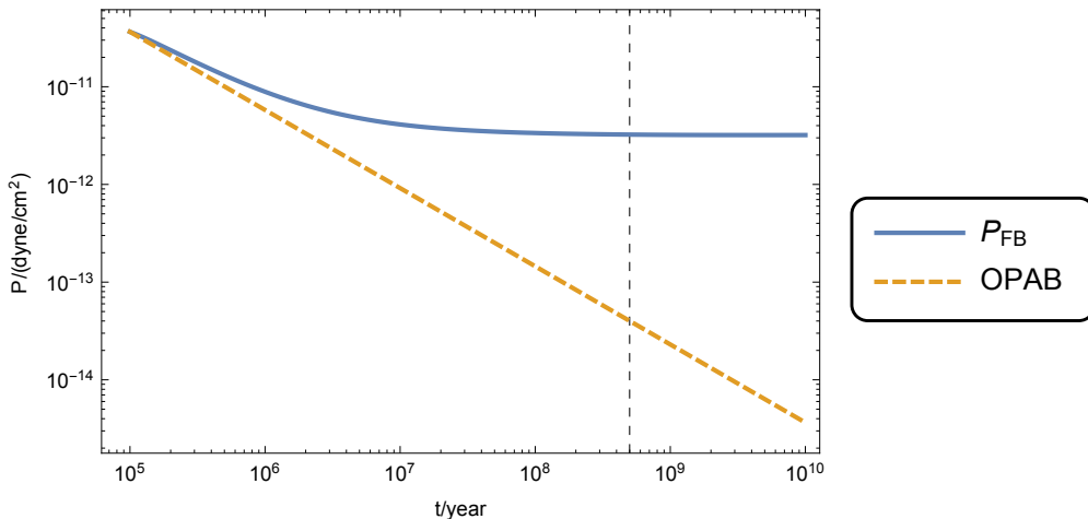
Fig. 6.— Pressure interior to the contact discontinuity (solid blue); this asymptotes to the assumed atmospheric pressure 3.2 \times 10^{-12} dyne \text{cm}^{-2} . Parameters as for Figure 4. The vertical line indicates when the bubble has attained a volume equivalent to the observed Fermi Bubbles (cf. Figure 4). The dashed orange curve is for an over-pressured, adiabatic bubble.
