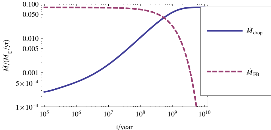
Fig. 7.— Mass drop out (solid blue) and mass growth of Bubbles (dashed purple). Parameters as for Figure 4. The vertical line indicates when the bubble has attained a volume equivalent to the observed Fermi Bubbles (cf. Figure 4). At times \gtrsim Gyr mass drop out by itself saturates the injection rate of freshly-heated plasma.
