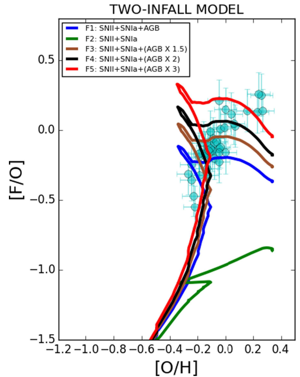
Fig. 1. Abundance ratio [F/O] as a function of [O/H] in the solar neighborhood for the two-infall chemical evolution model adopting various prescriptions for the channels of the fluorine production. For oxygen we use the Romano et al. (2010; model 15) prescriptions. The blue line represents the model F1 of Table 2, where fluorine is assumed to be produced by both AGB stars, SNe Ia, and SNe II. The green line indicates the model F2 (contributions to fluorine production only from SNe Ia and SNe II). The models F3, F4, and F5 in which the AGB yields are multiplied by factors of 1.5, 2, and 3, respectively (along with SN Ia, SN II channels) are indicated with brown, black, and red lines. Observational data by Jönsson et al. (2017a) are indicated with cyan circles.
