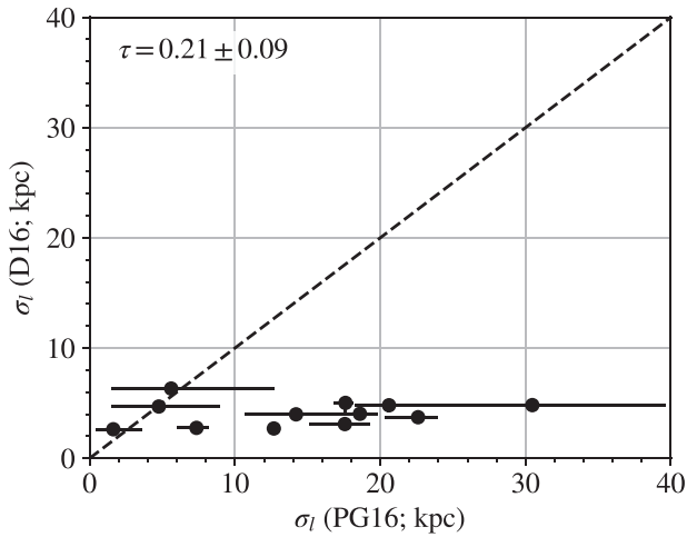
Figure 8. Comparison between kernel length scales derived using the Dopita et al. (2016) or the Pilyugin & Grebel (2016) ScI metallicity calibration. The 1:1 relationship is shown as a dashed black line. Kendall’s \tau correlation coefficient is shown in the top left. Typically, the kernel length scales derived from the Dopita et al. (2016) are significantly shorter, and reflect the higher scatter in this metallicity calibration, which the GPR models as significant variation over short scales.
