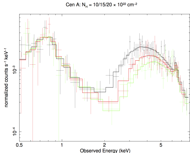
Fig. 28 Simulated SXI spectra of Cen A. THESEUS SXI can track fluctuations in line-of-sight column density N_{\text{H}} as density variations in its clumpy torus drift across the line of sight. Shown here are spectra corresponding to columns of 10, 15, and 20 \times 10^{22} \text{ cm}^{-2} , (black, red, and green, respectively, based on variations observed by [287]), each 70 ks accumulated exposure.
