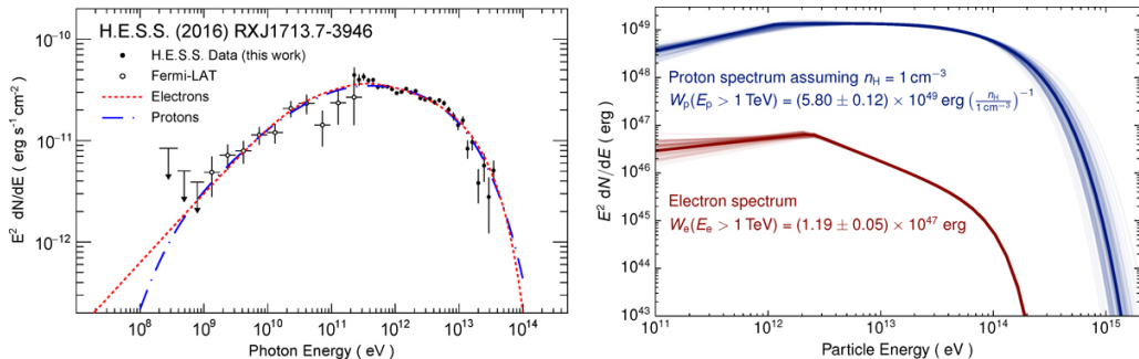
FIGURE 2. Left Panel: The black data points represent the measured X-ray (Cassam-Chenaï et al. 2004), GeV (Fermi-LAT) and TeV (H.E.S.S.) spectral energy distribution of the radiation from the shell of RX J1713.7-3946. The lines represent the multi-wavelength spectra predicted by NAIMA Zabalza (2015), assuming either a leptonic or hadronic origin of the emission. Right Panel: The spectral energy distributions of the electrons and protons producing the leptonic and hadronic emissions shown on the left panel.
