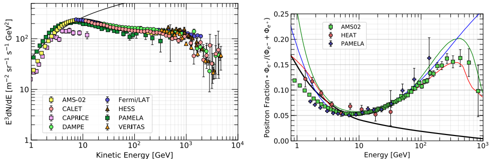
FIGURE 4. Left Panel: Differential spectrum of electrons and positrons multiplied by E^3 . Cosmic-ray electrons can be measured using space-born instruments such as AMS or Fermi-LAT up to 1 \sim \text{TeV} and CALET or DAMPE up to \sim 10 \text{ TeV} . Ground-based Cherenkov telescopes, such as H.E.S.S., MAGIC and VERITAS, which benefit from very large effective areas, have measured the flux up to 20 \text{ TeV} . The black line shows the proton spectrum multiplied by 0.01 (Shikaze et al. 2007). Right Panel: Positron fraction. Not all experiments are able to measure the electrons and positrons separately. Here measurements by Aguilar et al. (2019a); Adriani et al. (2009c); Beatty et al. (2004) are reported, together with a number of model predictions: the black curve is for pure secondary production in the standard scenario (Moskalenko & Strong 1998); the blue one includes a more sophisticated propagation model (Gaggero et al. 2013); the green one invokes dark matter decay (Ibarra et al. 2013); the red one includes a contribution from pulsars (Yin et al. 2013). The Figure is from Particle Data Group et al. (2020).
