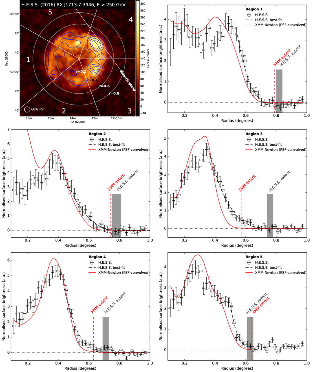
FIGURE 1. Top left panel: H.E.S.S. gamma-ray skymap of RX J1713.7-3946 (Aharonian et al. 2004; H. E. S. S. Collaboration et al. 2018). In blue the contours of the shell as observed by XMM in X-rays (Cassam-Chenaï et al. 2004). The morphology of the TeV shell resembles closely the X-ray shell. Top right panel and following; radial profiles of the emission at selected places along the shell from H.E.S.S. and XMM-Newton. In four out of five regions of the shell, the TeV supernova remnant is more extended than the X-ray one as a result of possible escape of high energy particles from the shell. The coordinate "Radius", used for the one-dimensional profiles, refers to the mean radius "r" of the shell over which average is performed.
