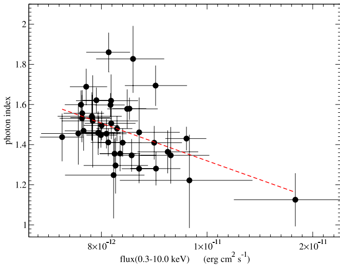
Figure 8. Scatter plot of the flux in 0.3–10.0 keV range vs. the X-ray photon index ( \alpha_X ). The dashed lines represent a linear best fit model. Using the Monte Carlo method described in Section 2.2.1, we get a correlation coefficient r = -0.31 with a 95% confidence limit of -0.55 \leq r \leq -0.05 . (A color version of this figure is available in the online journal.)
