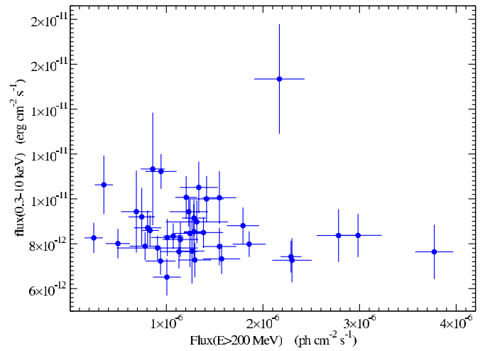
Figure 10. Scatter plot of the XRT flux in the 0.3–10 keV band vs. the Fermi -LAT flux ( E > 200 MeV). (A color version of this figure is available in the online journal.)
