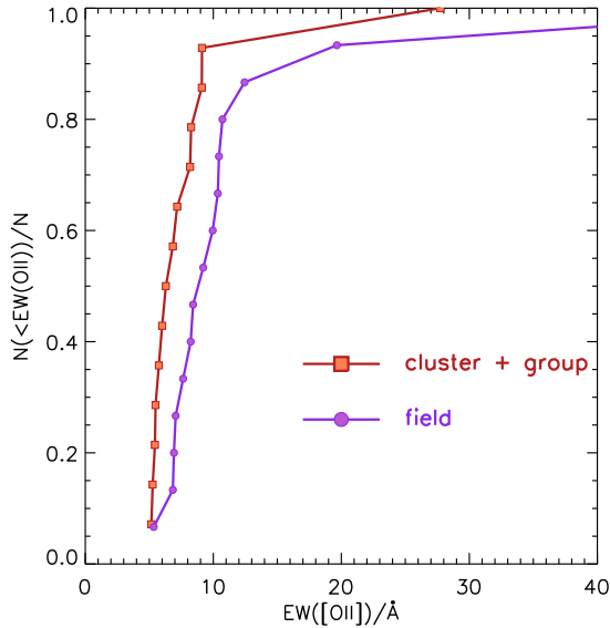
Figure 8. The cumulative distributions of \text{EW}([\text{O II}]) for galaxies with \text{EW}([\text{O II}]) > 5 \text{ \AA} that are classified as “older” based on D_n(4000) and the (\text{H}\delta_{\text{abs}}/\text{H}\gamma_{\text{abs}}) strength. The cluster+group distribution is shifted towards lower \text{EW}([\text{O II}]) values, with only a 3% K-S probability of being drawn from the same distribution as the field galaxies.
