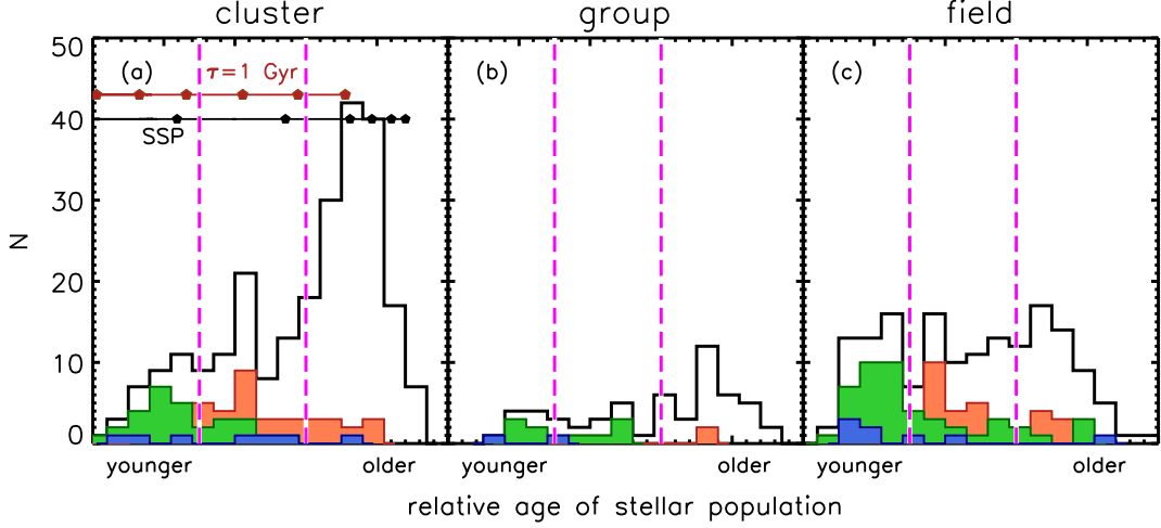
Figure 2. A histogram of galaxies along the direction of the sequence in \langle H\delta_{abs}H\gamma_{abs} \rangle and D_n(4000) (Fig. 1.) The x-axis corresponds to the shortest distance of each object in Fig. 1 to a zeropoint line in the far upper left of the panels in that plot that has an identical slope to the magenta lines shown in that figure. The units are arbitrary but identical in each plot. The different panels correspond to cluster, group, and field galaxies. The vertical lines mark the bins in relative stellar population age that we label “older” (right bin), “intermediate” (middle bin), and “younger” (left bin). They are identical to the magenta lines shown in Fig. 1. The colored histograms in each panel show the distribution of galaxies with EW([O II]) > 5\text{\AA} using the same color coding by emission line strength as in Fig. 1. The horizontal lines in panel (a) correspond to the single burst (black) and exponential model with \tau = 1\text{Gyr} (red) shown in Fig. 1. The points on those lines mark 1 Gyr intervals increasing to the right.
