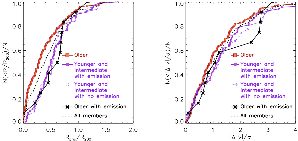
Figure 10. Left panel – The cumulative histogram of R_{proj}/R_{200} for the different galaxy populations. All galaxies with emission are systematically biased to large cluster-centric radii. Right panel – The cumulative histogram of |\Delta v|/\sigma for the same galaxy populations. All of the populations are statistically consistent with being drawn from the same underlying distribution.
