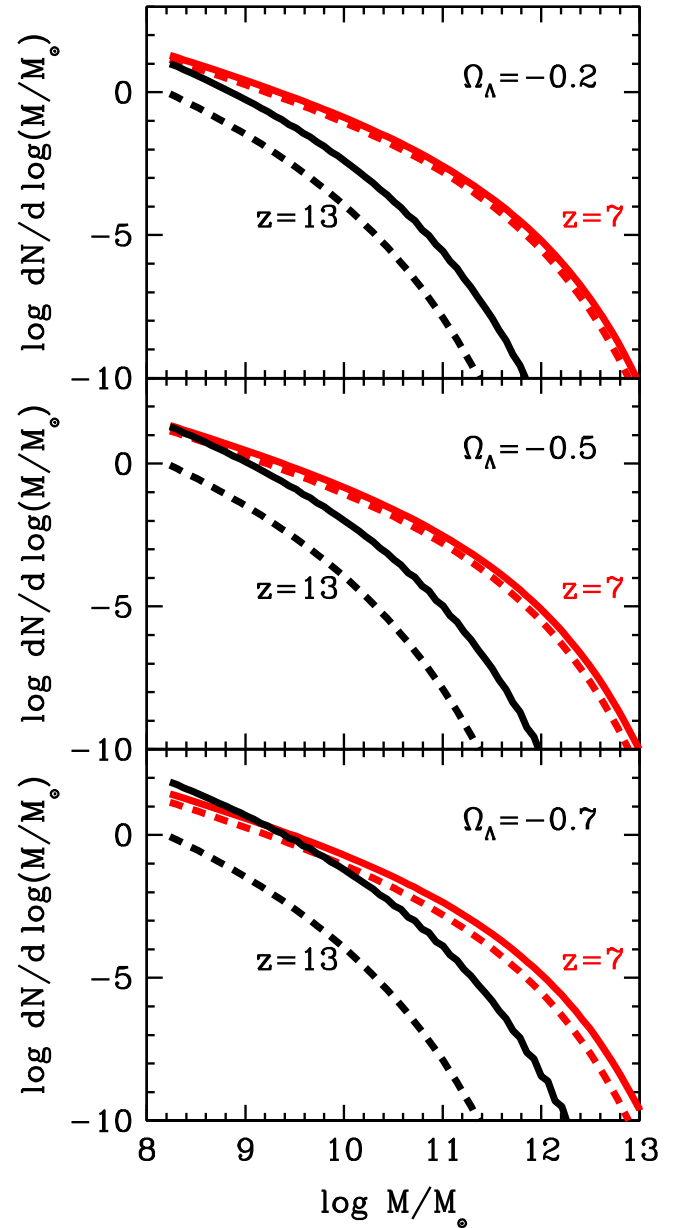
Figure 2. The DM halo mass function corresponding at redshift z = 7 (red lines) and z = 13 (black lines) in nCC models with different, negative values of \Omega_\Lambda are shown as continuous lines. For reference, we also show as dashed lines the halo mass function corresponding to the standard \Lambda CDM cosmology.
