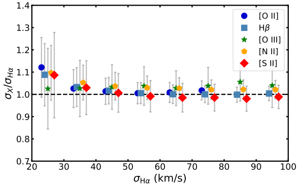
Figure 16. Ratio between H\alpha velocity dispersion and velocity dispersions of [O\text{ II}] \lambda 3727 , H\beta , [O\text{ III}] \lambda 5008 , [N\text{ II}] \lambda 6584 , and [S\text{ II}] \lambda 6717 as a function of \sigma_{H\alpha} . For each emission line the sample is limited to star-forming spaxels for which both H\alpha and the other emission line are detected with \text{SNR} > 50 . Filled points show the sigma-clipped mean of the distribution while the error bars indicate the 1\sigma width of the observed distribution (uncertainties in the mean are smaller than the symbols).
