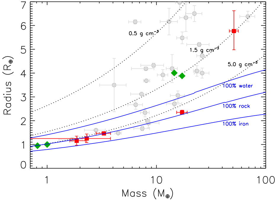
Fig. 1. Mass-radius diagram of the known transiting planets with radius R_p \leq 7 R_\oplus , mass M_p \leq 100 M_\oplus , and precision on the mass better than 30%. Green diamonds indicate Neptune, Uranus, the Earth, and Venus (from right to left). The three dotted lines indicate isodensity curves of 0.5 , 1.5 , and 5 \text{ g cm}^{-3} , and the blue solid lines show the mass and radius of planets consisting of pure water, 100% rocks, and 100% iron Seager et al. (2007). The positions of the Kepler planets characterized with HARPS-N to date are shown with red squares.
