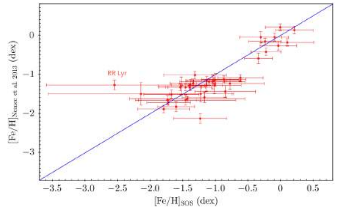
Fig. 20. Comparison of the photometric metallicities derived by the SOS Cep&RRL pipeline and the metallicities from high-resolution spectra of 39 RR Lyrae stars of the Nemec et al. (2013) calibrators.
