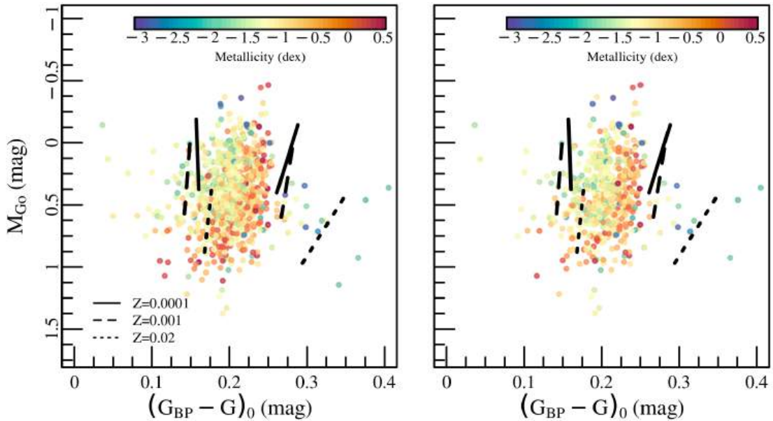
Fig. 29. HR diagram in G absolute magnitude ( M_{G_0} ) and dereddened (G_{BP} - G)_0 colour. Left panel: M_{G_0} (G_{BP} - G)_0 CMD of 915 DR3 RRab stars that have \sigma_w/w < 0.1 , RUWE < 1.4 , and A(G) < 0.2 ; right panel: same as in the left panel, but for 620 RR Lyrae of the sample for which A(G) < 0.1 . The sources are colour-coded according to their metallicity. The lines show the boundaries of theoretical ISs for RRab stars of three different chemical compositions ( Z = 0.0001 , solid lines; Z = 0.001 , dashed lines; and Z = 0.02 , dotted lines) from Marconi et al. (2015).
