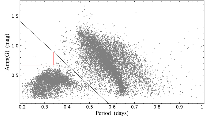
Fig. 3. New boundaries of the RRAb and RRC regions in the PA diagram defined by a sample of about 15 000 RR Lyrae stars that was randomly selected from the final RR Lyrae catalogue published in the dr3_vari_rrlyrae table of Gaia DR3. The dotted portion of the black line separating RRAb from RRC stars was replaced by the broken red line in order to properly classify high-amplitude RRAb stars with pulsation periods in the same domain as RRC stars (see text for details).
