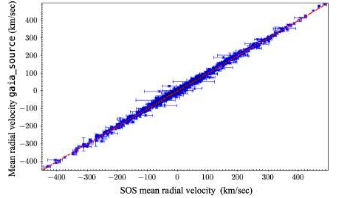
Fig. 16. Comparison of the mean RV values in the DR3 vari_rrlyrae table, which are computed with the SOS Cep&RRL pipeline from the modelled RV curves of the RR Lyrae stars, and the combined RV values in the DR3 gaia_source table for the 1054 RR Lyrae stars for which both values are available. The median and mean difference between the two average values is 5.21 and 6.88 km s -1 (with a standard deviation of 6.35 km s -1 ), respectively.
