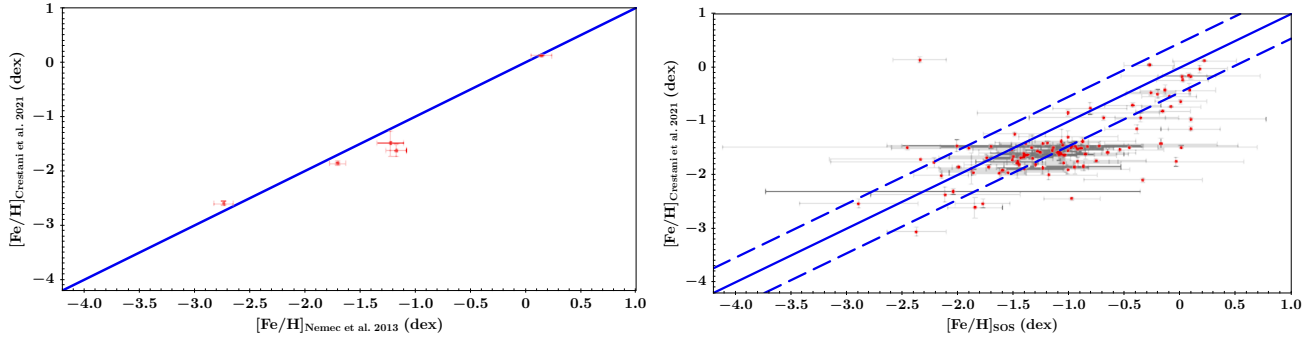
Fig. 21. Left panel: comparison of the metallicity from high-resolution spectra for five RR Lyrae stars in common in Nemec et al. (2013) and Crestani et al. (2021). Right panel: comparison of the photometric metallicities derived by the SOS pipeline and the spectroscopic metallicities from high-resolution spectra derived by Crestani et al. (2021) for 105 RR Lyrae stars in common in the two samples. The two dashed lines are offset by \pm 0.46 dex, the mean error of the photometric metallicities (see Fig. 19), from the one-to-one line.
