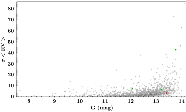
Fig. 14. Uncertainty of the mean RV values as a function of the SOS mean \langle G \rangle magnitude for 1097 out of 1100 RR Lyrae stars (filled grey points). We plot in different colours one DCEP (red symbol) and three ECLs (green symbols) that contaminate the 1097 RR Lyrae sample (see Sect. 6 for details).
