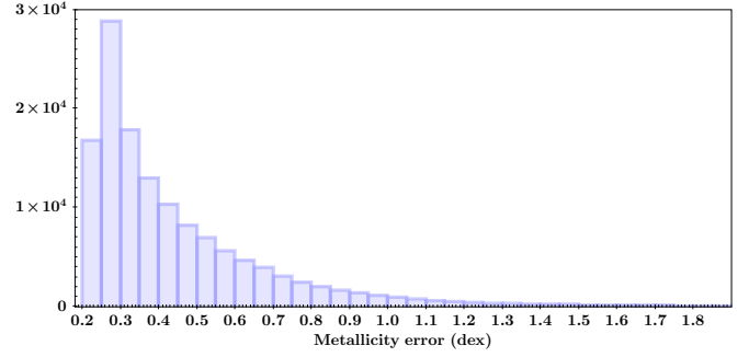
Fig. 19. Error distribution of the metallicities derived for 133 557 DR3 RR Lyrae stars by the SOS pipeline. The mean and median metallicity errors are 0.46 dex (0.33 dex std) and 0.36 dex, respectively. We show only sources with \sigma_{[\text{Fe}/\text{H}]} \leq 2.0 dex (i.e. 99.6% of the sample). We also note that for 71% of the sources in the plot, \sigma_{[\text{Fe}/\text{H}]} \leq 0.5 dex.
