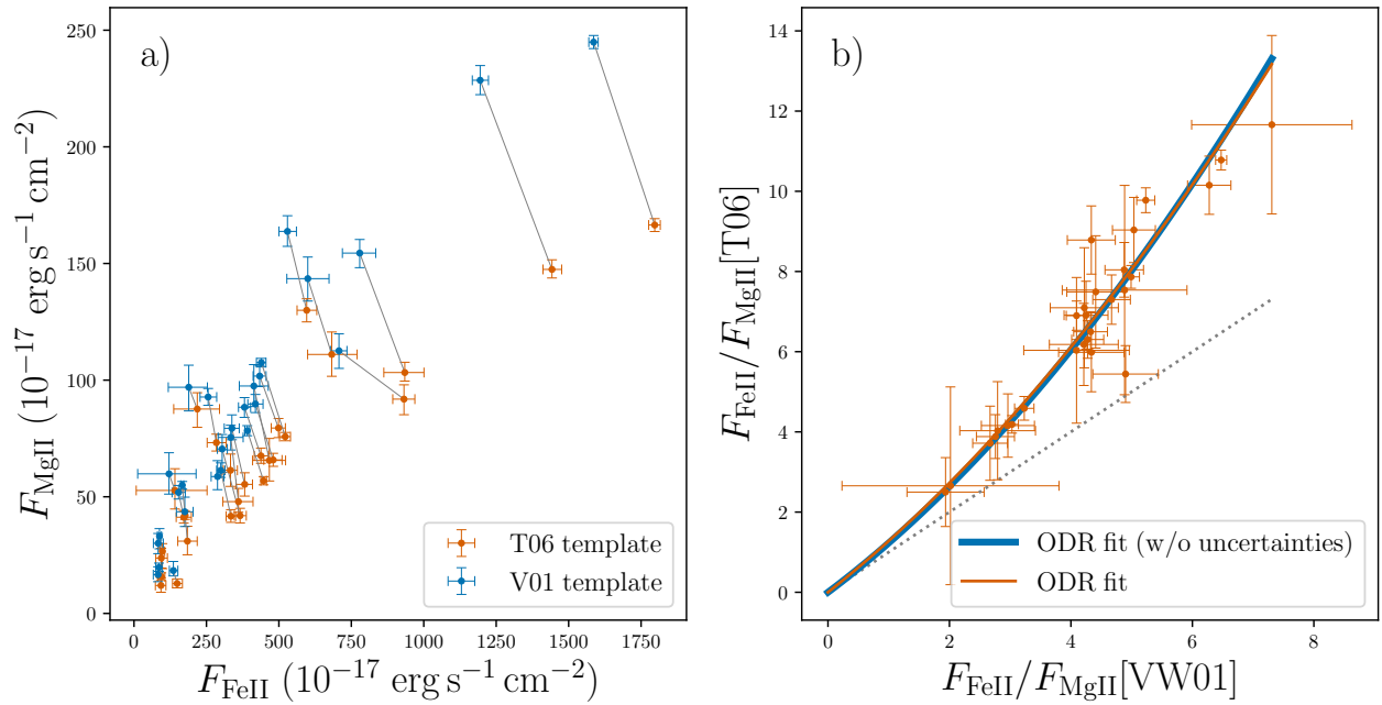
Figure 8. Influence of the iron template on the F_{\text{FeII}}/F_{\text{MgII}} ratios. a) : Mg II flux as a function of Fe II flux. The change from the T06 (orange) to the V01 (blue) template introduces a diagonal shift (grey line) of the data points toward lower Fe II and higher Mg II flux. b) : A comparison between the flux ratios calculated with both templates. We show our best fit using orthogonal distance regression as the orange solid line. The solid blue line shows the same fit excluding the measurement errors. The F_{\text{FeII}}/F_{\text{MgII}} ratio data based on the T06 template clearly lie above the 1:1 relation (grey dotted line).
