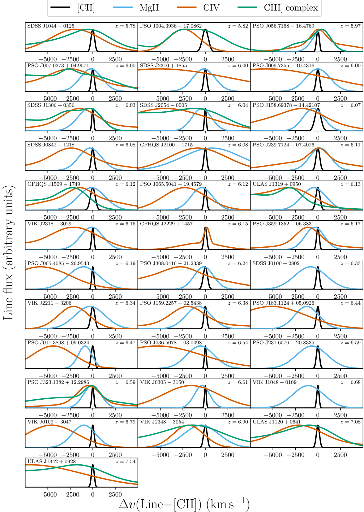
Figure 10. Line models fit to the CIII ], CIV and MgII broad emission lines in comparison to the Gaussian line fits of [C II] line from mm observations for each quasar. We adopted the [C II] redshift as the systemic redshift and normalized the peak flux of all lines for a better visual comparison between the line widths and velocity shifts. The figure highlights the accuracy of the [C II] redshift with respect to the broad UV emission lines.
