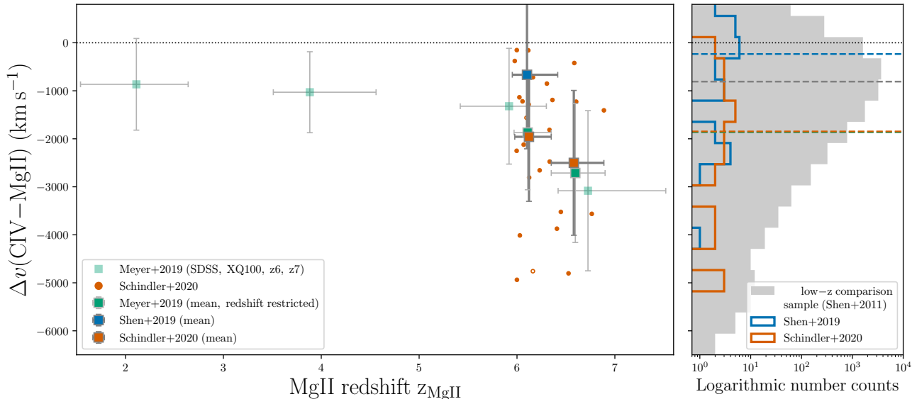
Figure 11. Left panel: CIV-MgII velocity shifts of individual high-redshift quasars as a function of the MgII redshift. Our results are shown in orange. We calculate the mean (orange square) and standard deviation (dark grey error bars) CIV-MgII for two sub-samples split at z = 6.35 . The error bars in the redshift direction show the redshift bin. We contrast these results with the mean results of the samples of Meyer et al. (2019) (light green squares). For an appropriate comparison we restrict the z6 and z7 Meyer et al. (2019) samples to the same redshift ranges as our sample and re-compute the mean (green squares), yielding very good agreement with our data. All velocity shift measurements are based on the peak redshifts of the emission lines. Right panel: Logarithmic CIV-MgII velocity shift histograms. We compare our results (orange) to the high-redshift sample of Shen et al. (2019a) (blue). Both measurements are contrasted with low redshift data from Shen et al. (2011) at 1.5 \leq z \leq 2.2 and restricted to \log(L_{\text{bol}}/\text{erg s}^{-1}) = 46.5 - 47.5 for a valid comparison to the high redshift quasars. The colored dashed lines show the median of the three distributions as well as the combined z6 and z7 samples of Meyer et al. (2019) (green).
