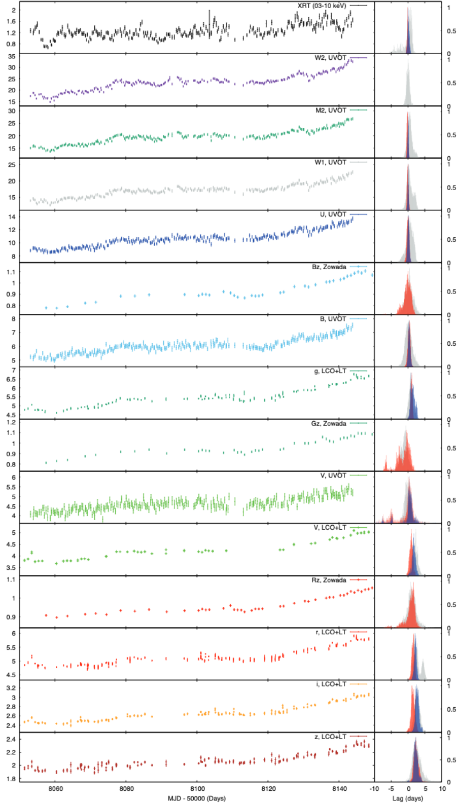
Figure 2. Left-hand panels: Light curves used for the short time-scale lag analysis. While the XRT light curve is shown in count \text{s}^{-1} , the measurements in the UVOT filters are in (\times 10^{-15}) \text{ erg cm}^{-2} \text{ s}^{-1} \text{ \AA}^{-1} . Regarding the ground-based observations, LCO + LT is in (\times 10^{-15}) \text{ erg cm}^{-2} \text{ s}^{-1} \text{ \AA}^{-1} , while RGB Zowada light curves are in arbitrary units. Right-hand panels: Lag versus UVW2 band probability distribution using unfiltered light curve (grey), and filtered ones by removing the linear trend (red) and a 10-d box-car moving average (blue).
