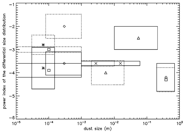
Fig. 7 Power index of the differential size distribution of 67P/C-G. Dotted lines: power index before the 2015 equinox. Continuous lines: power index after the 2015 equinox, up to just after the 2015 perihelion. The ranges along the x axis show the instrument sensitivity, the ranges along the y axis are given by the uncertainty of the power index. Stars: COSIMA data (Merouane et al. 2017). Diamonds: GIADA data (Rotundi et al. 2015; Fulle et al. 2016c). Triangles: OSIRIS observations of single particles in the coma (Rotundi et al. 2015; Fulle et al. 2016c; Ott et al. 2017). Dotted diamond: OSIRIS observations of pebbles in Sais (Pajola et al. 2017a). Dotted square: ROLIS observations of pebbles in Agilkia (Pajola et al. 2017a). Squares: Ground-based observations, tail models (Moreno et al. 2017). Crosses: Ground-based observations, trail models (Moreno et al. 2017)
