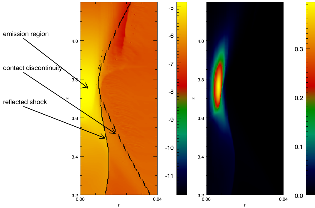
Fig. 2. The left panel shows the pressure distribution in the region marked by the red rectangle in Fig. 1 for the case with \xi_c = 0.01 . The arrows indicate the main features already displayed in Fig. 1. The right panel displays the distribution of the observed emissivity (see Eq. (17))
